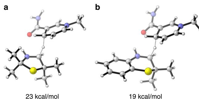
Fig. 6 DFT studies. Transition states obtained by DFT calculations for the reduction of the non-substituted protonated 3-thiazoline ( a ) and protonated 2H-1,4-benzothiazine ( b ) by means of a dihydropyridine mimic as a reducing agent (Gibbs free energies of activation \Delta G_{298\text{K}} are given)
