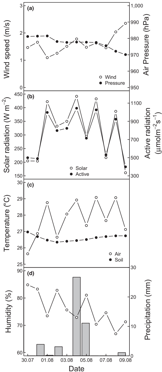
FIGURE 2 Daily meteorological average values before, during and after the experiment: Panel (a) daily wind speed (m/s), daily atmospheric pressure (hPa); Panel (b) day time ( W/m^2 ) average solar radiation and photosynthetically active radiation (PAR, \mu mol\ m^{-2}\ s^{-1} ); Panel (c) daily average air and soil temperature at 20 cm soil depth ( ^{\circ}C ); Panel (d) daily averaged air humidity (RH, %) and total daily precipitation (mm). Measurements started on the 4th of August (later referred as day 1) before the rain event (night between 4th and 5th of August) and were continued until the 7th of August
