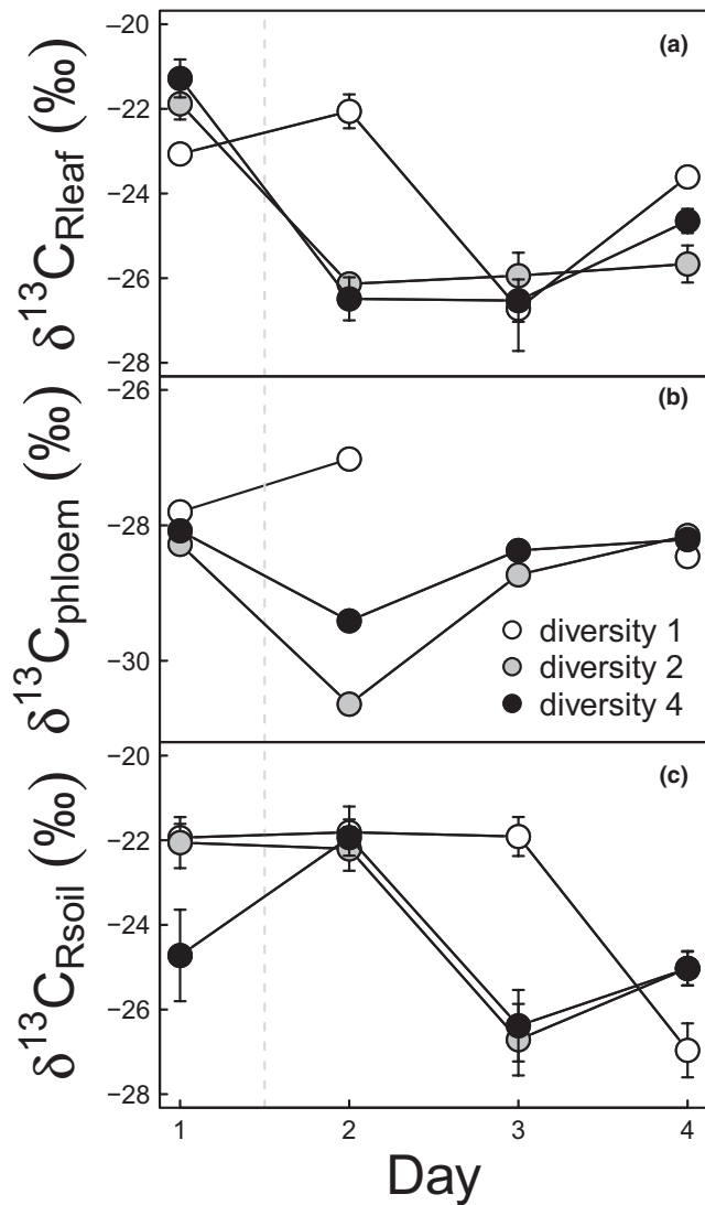
FIGURE 4 Response of \delta^{13}\text{C} values of leaf-respired \text{CO}_2 ( \delta^{13}\text{C}_{\text{Rleaf}} ‰, panel a), phloem organic matter ( \delta^{13}\text{C}_{\text{phloem}} ‰, panel b) and soil-respired \text{CO}_2 ( \delta^{13}\text{C}_{\text{Rsoil}} ‰, panel c) of Lithocarpus glaber to a precipitation event in plots with different diversity: monoculture (diversity 1), two-species mixture (diversity 2) and four-species mixture (diversity 4). The dashed line represents the rain event that took place between day 1 and 2. Each point represents the average value ( n \geq 3 ) for a given diversity level on a given day, except for phloem ( n = 1 ). Error bars indicate \pm 1 SE
