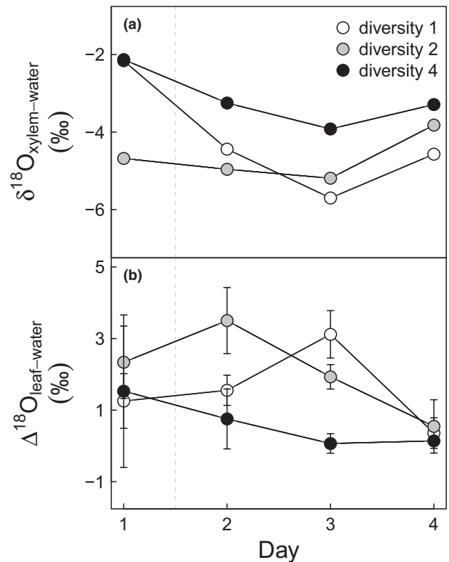
FIGURE 5 Response of xylem-water \delta^{18}\text{O} (‰, panel a) and leaf-water \Delta^{18}\text{O} (‰, panel b) of Lithocarpus glaber to a precipitation event in plots with different diversity: monoculture (diversity 1), two-species mixture (diversity 2) and four-species mixture (diversity 4). The dashed line represents the rain event that took place between day 1 and 2. Each point represents the average value ( n \geq 3 ) for a given diversity level on a given day. Error bars indicate \pm 1 SE (there is no error bar for xylem water \delta^{18}\text{O} , see text)
