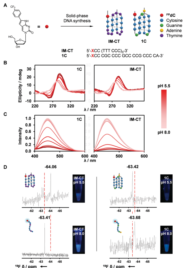
Fig. 2 Characterization of FPdC -containing i-motif structures. (A) I-Motif-forming DNA sequences, 1C and IM-CT, containing FPdC . (B) CD and (C) normalized fluorescence spectra of 1C and IM-CT with pH. (D) 19 F NMR spectra and images of 1C and IM-CT.
