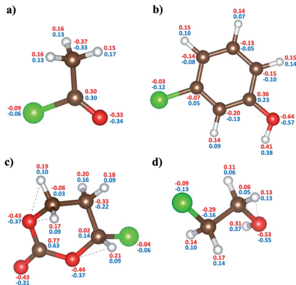
Fig. 5 The comparison of charge distributions of DFT and ReaxFF in (a) C_2H_3ClO , (b) C_6H_5ClO , (c) C_4H_5ClO_3 , and (d) C_2H_5ClO . The red-colored values are for DFT-calculated Mulliken charges and the blue-colored values are for the ReaxFF-calculated EEM charges based on electronegativity. The brown, red, white, and green-colored balls indicate C, O, H, and Cl atoms, respectively.
