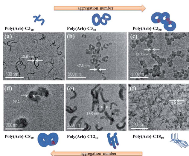
Fig. 6 TEM images of (a) poly(Arb)-C 3 10 , (b) poly(Arb)-C 3 30 , (c) poly(Arb)-C 3 50 , (d) poly(Arb)-C 8 10 , (e) poly(Arb)-C 12 10 , and (f) poly(Arb)-C 18 10 , and their plausible aggregated structures.
