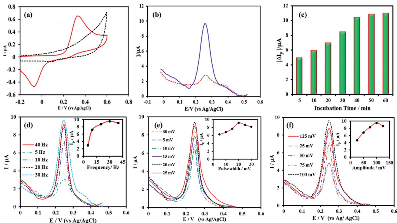
Fig. 4 (a) Cyclic voltammograms of the aptamer functionalized NPG electrode in 0.02 M PBS (pH 5.5) at a scan rate of 50 mV s -1 before (dashed, black line) and after DHBA immobilization (solid, red line), (b) SWV curves obtained for the proposed aptasensor in 0.02 M PBS, pH 5.5, before (dashed, red line) and after challenging with 1 μM cocaine (solid, blue line), the effect of incubation time (c), frequency (d), pulse width (e) and amplitude (f) on the SWV response of the aptasensor toward cocaine.
