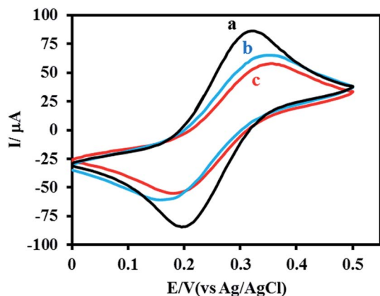
Fig. 3 Cyclic voltammograms of 0.5 mM of [Fe(CN) 6 ] 3-/4- in 0.1 M PBS, pH 5.5, containing 0.1 M KCl at a scan rate of 50 mV s -1 obtained for electrodes at different assembly steps: flat gold (a), NPG (b) and aptamer functionalized NPG electrode before (c) and after immobilization with DHBA redox probe.
