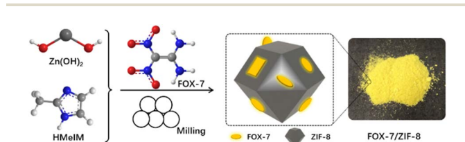
Scheme 1 Synthesis route for FOX-7/ZIF-8 composites.
