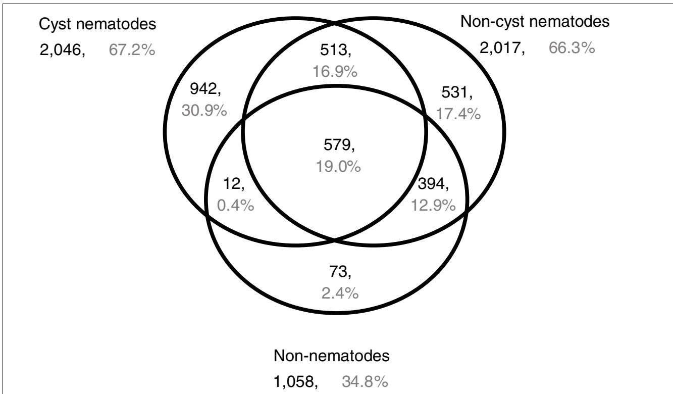
Figure 1 Venn diagram showing distribution of H. glycines BLAST hits by database. Forty-four percent of all 6,860 H. glycines contigs matched sequences in at least one of three databases at a threshold value of 1 \times 10^{-20} : (a) All cyst nematodes without H. glycines . (b) All non-cyst nematodes. (c) All non-nematodes.
