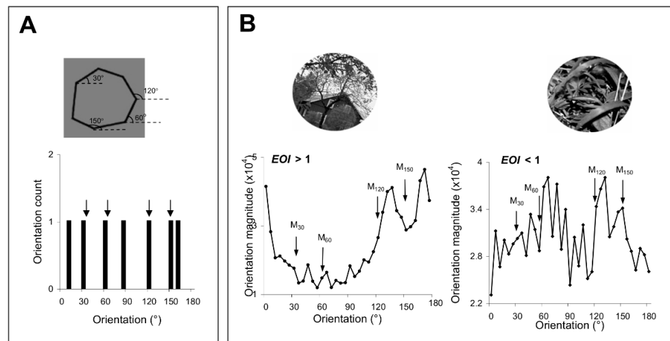
Figure 2. (A) Shape discrimination. We generated polygons with four of the sides oriented along the exposed axes, i.e., 30°, 60°, 120°, and 150°. The histogram below indicates the orientation distribution of the corresponding shape, with arrows pointing toward the orientations presented during the exposure stage. (B) Image discrimination. Two representative images and their corresponding exposure orientation index, EOI, which quantifies the relative strength of the orientation signals along exposed axes in each image. For each image, we determined the orientation at each pixel location based on the direction of the local gray-scale gradient in a standard 25-pixel array from the arc tangent of the partial derivative of brightness in a 5 \times 5 kernel in the vertical direction, divided by this value in the horizontal direction [13]. The results for all the pixels are represented as orientation magnitude histograms (below each image). Arrows point toward the orientations presented during exposure.
