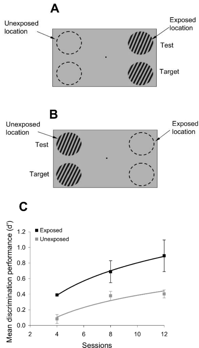
Figure 5. Simultaneous orientation discrimination. (A,B) Orientation discrimination performance was measured at both the exposed (A) and unexposed (B) locations by simultaneously presenting the test and target stimuli. The test was always presented at a fixed location (above the unexposed location). The center-to-center distance between the target and test locations was 5^\circ . Each discrimination test was conducted after an exposure session similar to that discussed in Figure 1. (C) Exposure to orthogonal orientations significantly alters simultaneous orientation discrimination performance at the exposed location.
