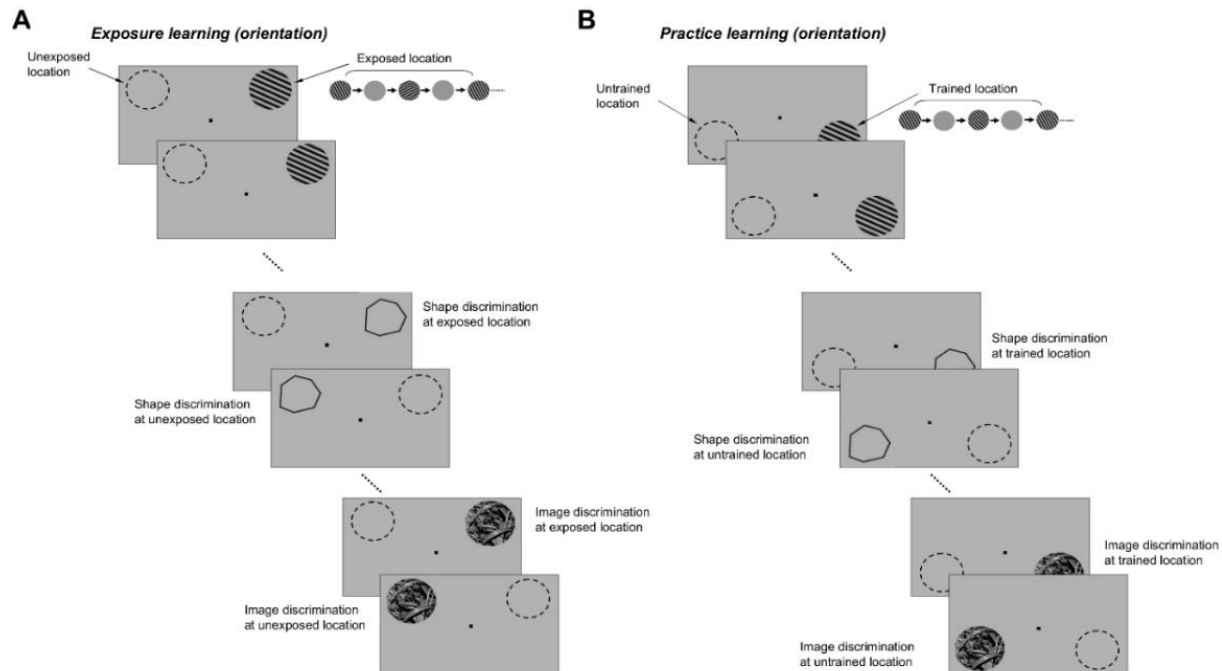
Figure 7. Stimulus generalization experiments. (A) Exposure learning. Subjects were successively exposed to two pairs of orthogonal orientations, 60°/150° and 30°/120°, 12 sessions for each pair. After completion of the orientation exposure sessions, subjects were required to discriminate shapes and natural scenes. Discrimination tests were performed at both exposed and unexposed locations by successively flashing shapes or natural images that were slightly tilted relative to each other. (B) Practice learning. At another spatial location, subjects practiced orientation discriminations around the four orientations used in the exposure experiment (12 sessions per orientation). After the completion of the orientation discrimination practice sessions, subjects were required to discriminate shapes and natural scenes at both the trained and untrained locations.
