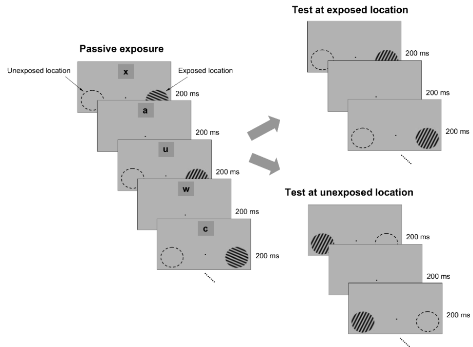
Figure 1. Exposure paradigm. The exposure phase consisted of successive presentations of specific orientations ( 3^\circ circular sine-wave gratings) that were flashed for 200 ms each at an exposed location for several minutes. Exposure was performed only at the exposed location, while another, unexposed, location was not stimulated. Throughout the exposure stage, a letter identification task (letters were located 7^\circ away from the fixation point) was paired with the exposure stimuli (each letter was flashed for 200 ms). At the end of the exposure session, subjects were required to recall how many times a specific letter occurred in the sequence. The exposure stage was followed by a delayed match-to-sample orientation discrimination task around the experienced orientations, conducted both at the exposed and unexposed locations. One stimulus (target grating) had an orientation that always matched the orientation of the exposed stimuli, whereas the second stimulus (test grating) had a random orientation that was within 5^\circ of the target. The target appeared first on 50% of the trials. At the end of each trial, subjects had one second to press a button whenever the target and test stimuli had a similar orientation.
