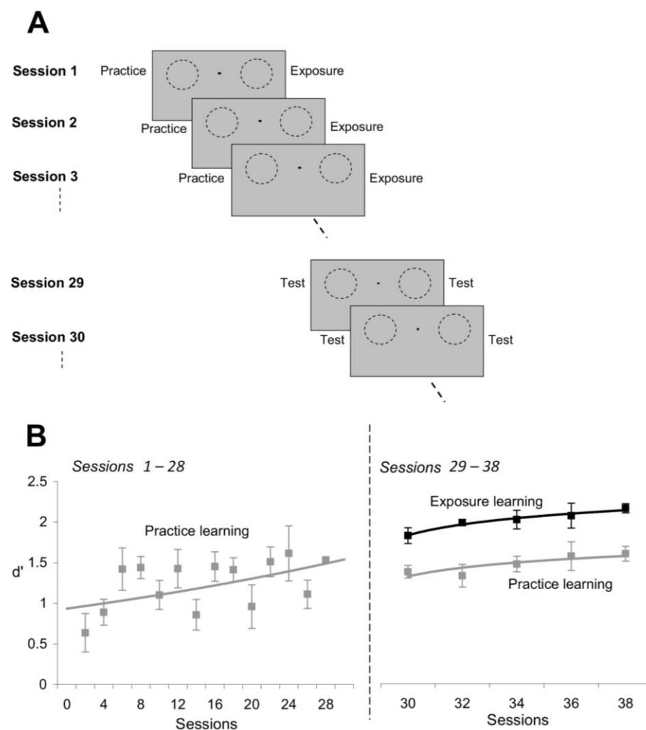
Figure 6. Exposure learning develops more rapidly than practice learning. (A) Experimental design. Subjects were required to experience practice learning at one location (left visual field) and exposure learning at another location (right visual field) for the same number of sessions (sessions 1 through 28). In sessions 29–38, orientation discrimination performance was measured at both exposed and unexposed locations to directly compare the effects of practice and exposure learning. (B) Exposure learning was stronger and developed more rapidly than practice learning. Black line: discrimination performance ( d' ) at the exposed location (exposure learning); gray line: discrimination performance at the unexposed location (practice learning). Error bars represent SEM.
