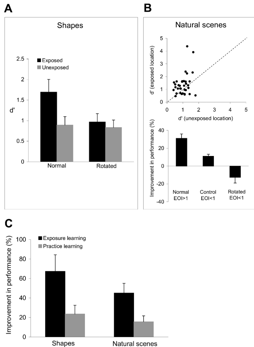
Figure 8. Results of the stimulus generalization experiments. (A) Shape discrimination performance is improved after exposure to orthogonal orientation sequences. In the ‘normal’ condition, i.e., shapes were not rotated, there is a significant improvement in shape discrimination performance only at the exposed location (black bars), whereas there is no improvement in performance at the unexposed location (grey bars). In the ‘rotated’ condition, we rotated the target and test polygons by 20^\circ , in which case the improvement in shape discrimination performance at the exposed location was abolished. (B) Top: Image discrimination performance is improved after exposure to orthogonal orientation sequences. The scatter plot represents the discrimination performance at the exposed location vs. that at the unexposed location. Each point represents the d' value for one subject and one image (averaged across 3 sessions). Only images with an exposure orientation index greater than 1 were included in the analysis. Bottom: Exposure to orthogonal orientations does not improve the discrimination of images with weak orientation signals along exposed axes ( EOI < 1 ) and the discrimination of images that were rotated by 20^\circ . We rotated only the images that had strong orientation signals along the exposed axes ( EOI > 1 before rotation). (C) Mean improvement in shape and image discrimination performance at the exposed and trained locations (relative to the unexposed and untrained locations). Subjects exhibited a larger mean improvement in shape and image discrimination performance after exposure learning (black bars) than after practice learning (grey bars). The improvement in discrimination performance was compared in 4 sessions at the exposed and trained locations in each subject. Error bars represent SEM.
