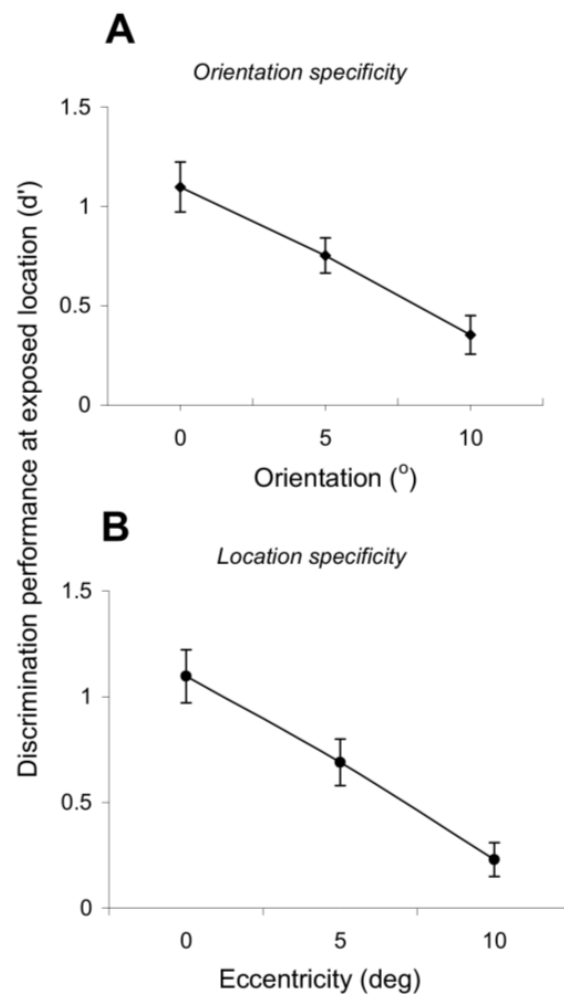
Figure 4. Specificity for orientation and retinal position. (A) Orientation specificity. The orientation discrimination performance at the exposed location gradually decreases as the test differs from the experienced orientations. Each point represents the mean performance (measured using d' ) obtained by averaging data across four test sessions when the target orientation was 5^{\circ} and 10^{\circ} away from the exposed orientations (exposure to 60^{\circ} – 150^{\circ} followed by tests at 65^{\circ} and 70^{\circ} ). (B) Position specificity. The orientation discrimination performance at the exposed location gradually decreases as the eccentricity at which the orientation discrimination test was performed increases. Each point represents the mean performance (measured using d' ) obtained by averaging data across four test sessions when the test location was 5 and 10^{\circ} away from the exposed location (exposure to 0^{\circ} eccentricity followed by tests at 5 and 10^{\circ} eccentricity on the horizontal axis). Error bars represent SEM.
