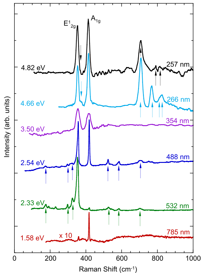
Figure 2. The Raman scattering spectra of monolayer WS 2 excited by 785, 532, 488, 354, 266, and 257 nm laser lines. The arrows denote the double resonance peaks.
