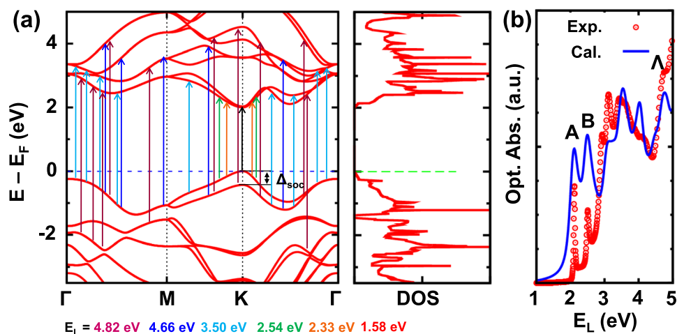
Figure 3. (a) Electronic band structure, density of states, and (b) optical absorption of monolayer WS 2 measured at 4.5 K. The labels A, B, and \Lambda denote A, B, and \Lambda excitons.
