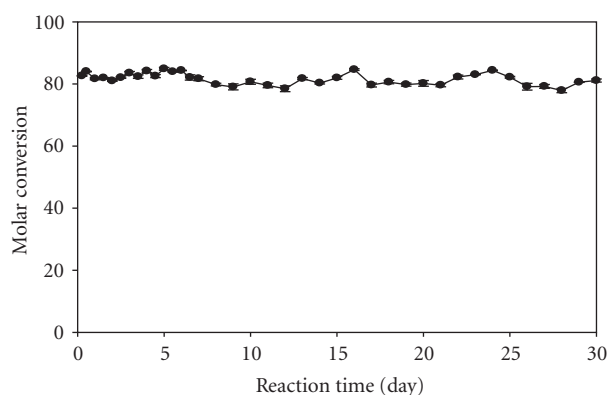
FIGURE 3: The effects of operating time on the conversion of soybean oil to biodiesel. Reaction conditions: temperature 52.1 ^{\circ}\text{C} , flow rate 0.1 mL/min, substrate molar ratio 1 : 4, and 1.7 g enzyme.
