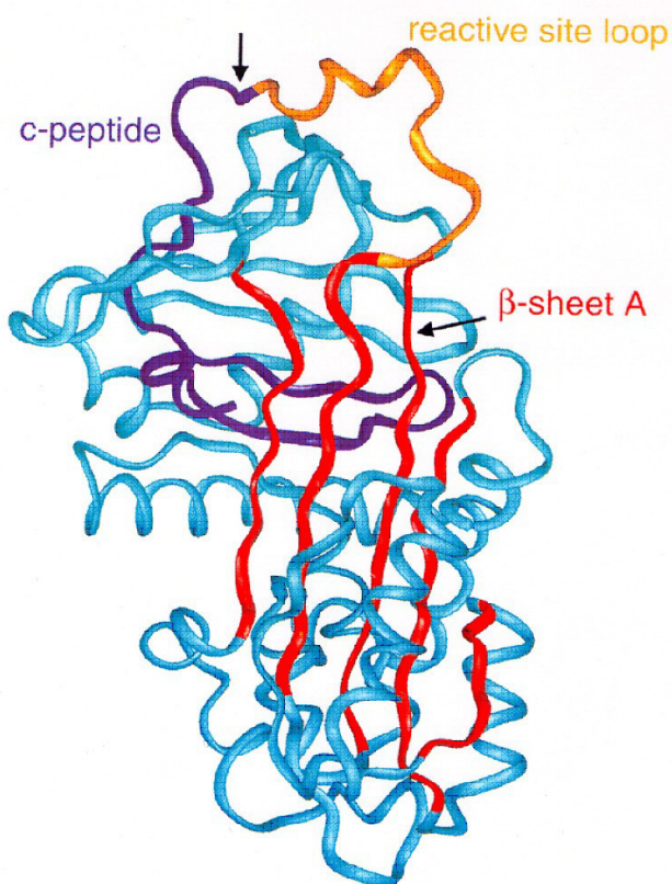
Figure 5 Structure of alpha-1-antitrypsin: 3 \beta -sheets and 8 \alpha -helices. The reactive loop site contains the neutrophil elastase binding site with a methionine residue. Reprinted from Janciauskiene S. Conformational properties of serine proteinase inhibitors (serpins) confer multiple pathophysiological roles. Biochim Biophys Acta , 2001, 1535:221-35. Copyright © 2001, with permission from Elsevier.
