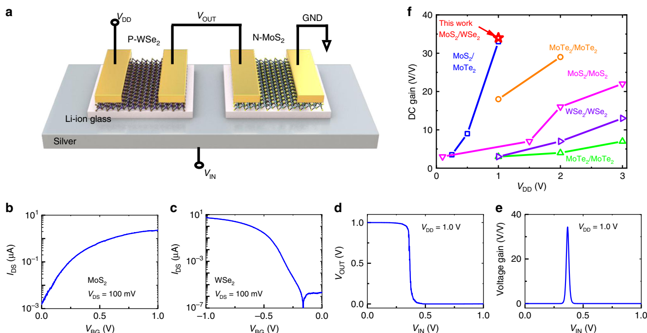
Fig. 4 CMOS inverter based on n-type MoS 2 and p-type WSe 2 FETs. a Schematic of a CMOS inverter with the drain of p-WSe 2 FET connected to the drain of n-MoS 2 FET. Transfer characteristics of b n-type MoS 2 FET. V_{TH} is -0.25 V. c p-type WSe 2 FET. V_{TH} is ~-0.50 V. d Output vs input voltage characteristics of the inverter. The mid-point voltage V_M is 0.38 V. Noise margin high ( NM_H ) and low ( NM_L ) as calculated from the graph are 0.56 V and 0.27 V, respectively. e Voltage gain vs. input voltage curve with a maximum gain of -34 at V_{IN} = 0.37 V. f DC gain vs. supply voltage ( V_{DD} ) of our n-MoS 2 /p-WSe 2 CMOS inverter (red) along with other CMOS inverters from the literature such as n-MoS 2 /p-MoTe 2 (blue) 60 , n-MoTe 2 /p-MoTe 2 (orange) 61 , n-MoS 2 /p-MoS 2 (magenta) 62 , n-WSe 2 /p-WSe 2 (violet) 63 , and n-MoTe 2 /p-MoTe 2 (green) 64 .
