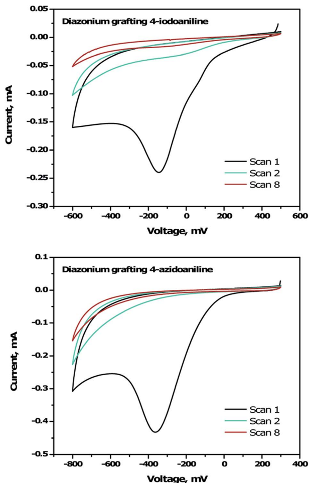
Fig. 2 Cyclic voltammograms showing the electrochemical grafting of in situ generated 4-iodobenzene diazonium chloride (top) and 4-azidobenzene diazonium chloride (bottom) on H-terminated B:NCD electrodes at a scan rate of 100 \text{ mV s}^{-1} for 8 scans.
