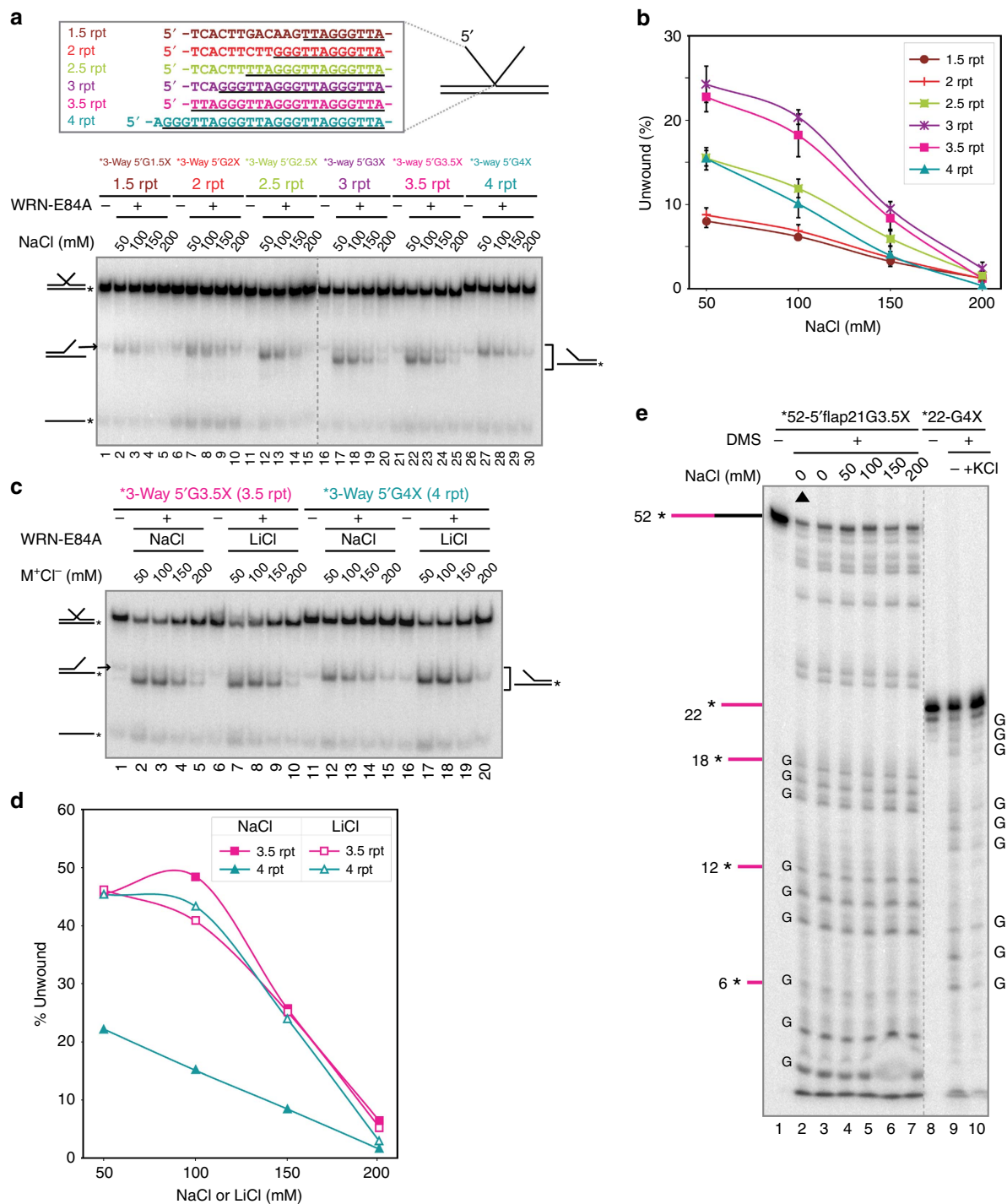
Figure 4 | WRN unwinding of strand invasion intermediates is enhanced by \geq 3 unstructured G-rich telomeric repeats on the invading strand. (a) Helicase assays performed with WRN-E84A (0.23 nM) incubated for 15 min with *3-way 5'G1.5X (1.5 repeats), *3-way 5'G2X (2 repeats), *3-way 5'G2.5X (2.5 repeats), *3-way 5'G3X (3 repeats), *3-way 5'G3.5X (3.5 repeats) or *3-way 5'G4X (4 repeats) substrate (0.2 nM each) in 50–200 mM NaCl as indicated. Migration positions of substrates and products are denoted. 5' flap sequences for substrates are shown (box), colour-coded in relation to a–d with G-rich telomeric sequence underlined. (b) Percent unwinding (mean \pm s.e.m. of three experiments, as in a). Asterisks indicate significant differences ( P < 0.04 , calculated using two-tailed unpaired Student's t -tests) of data points compared with analogous data points from each other substrate. (c) Helicase assays performed with WRN-E84A (0.27 nM) incubated for 15 min with *3-way 5'G3.5X (lanes 1–10) or *3-way 5'G4X (lanes 11–20) substrate (0.2 nM each) in 50–200 mM NaCl or LiCl as specified. Migrations of substrates and products are indicated. (d) Percent unwinding from each lane in c. (e) DMS protection assays were performed on *52-5'flap21G3.5X oligomer (0.2 nM) in 0–200 mM NaCl as specified and *22-G4X oligomer (0.2 nM) in 0 or 75 mM KCl. After denaturing PAGE, uncleaved oligos and fragments resulting from cleavage at DMS-methylated (unprotected) guanines are visualized; solid triangle (lane 2) indicates reaction was heat-denatured before DMS treatment. Fragments ending in guanines within telomeric repeats are denoted with 'G'; for reference, lengths of substrates and key DNA fragments (G-rich telomeric content in magenta) are indicated at the left.
