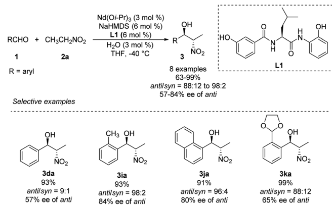
Scheme 4 Catalytic asymmetric anti -selective Henry reactions with Nd/Na/L1 heterobimetallic complex.
