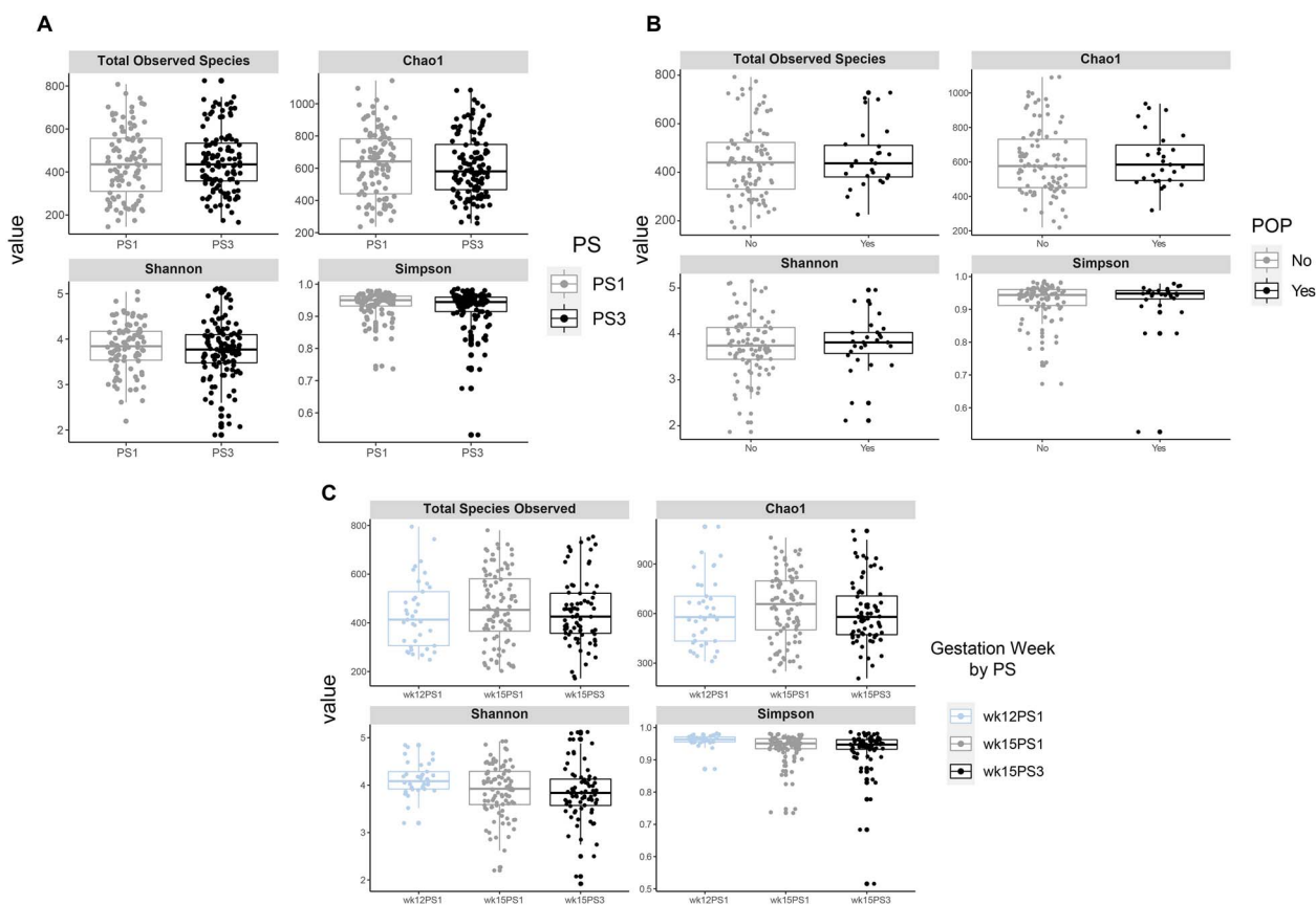
Figure 4. Alpha diversity of the vaginal microbiota for sows during late gestation. The above graphics compare alpha diversity measurements species evenness (Simpson), richness (TSO, Chao1), and diversity (Shannon) across the different variables within this study. (A) Alpha diversity measurements for sow vaginal microbiota at low (PS1; gray points, n = 101 ) or high (PS3; black points, n = 121 ) risk for POP at gestation week 15 (days 108–115). (B) Alpha diversity measurements for sows that subsequently did (Yes; black points, n = 28 ) or did not (No; gray points, n = 93 ) experience POP that also were scored PS3. (C) Alpha diversity measurements for sows from farm B at gestation week 12 scored PS1 (wk12PS1; light blue points, n = 39 ), gestation week 15 PS1 (wk15PS1; gray points, n = 61 ), and gestation week 15 PS3 (wk15PS3; black points, n = 78 ). Shannon and Simpson diversity were observed to be significantly different ( P \leq 0.03 ) with differences between week 12 sows and both week 15 PS1 and PS3 sows.
