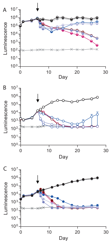
FIG 5 \text{D-Cycloserine} has similar effects on M. tuberculosis growth in 2D and 3D cultures. (A) M. tuberculosis growth in 7H9 broth. \text{D-Cycloserine} at a low concentration ( 20 \mu\text{g/ml} ) had a temporary effect on M. tuberculosis growth (light purple) similar to that of INH at 0.25 \mu\text{g/ml} (blue). \text{D-Cycloserine} at 200 \mu\text{g/ml} killed M. tuberculosis more rapidly than (dark purple) and as effectively as moxifloxacin (brown, 5 \mu\text{g/ml} ). Linezolid was the most effective second-line antibiotic (magenta, 24 \mu\text{g/ml} ). The diluent DMSO (gray) did not affect M. tuberculosis growth relative to that in 7H9 broth only (black). (B) M. tuberculosis growth in 2D PBMC cultures. \text{D-Cycloserine} at both concentrations inhibited M. tuberculosis growth (purple) more rapidly than the other antibiotics (moxifloxacin [brown, 5 \mu\text{g/ml} ], linezolid [magenta, 24 \mu\text{g/ml} ], and INH [blue, 0.25 \mu\text{g/ml} ]). Shown is M. tuberculosis growth in control samples (black) and with DMSO (gray). (C) M. tuberculosis growth in a 3D cell culture model. \text{D-Cycloserine} , linezolid, and moxifloxacin have an efficacy similar to that in a 2D cell culture (purple), while INH (blue) is more consistently bactericidal. Gray lines indicate background levels of luminescence. Black arrows indicate the day antibiotics were added. Data are the mean \pm the standard error of the mean of an experiment performed in triplicate and are representative of three separate experiments.
