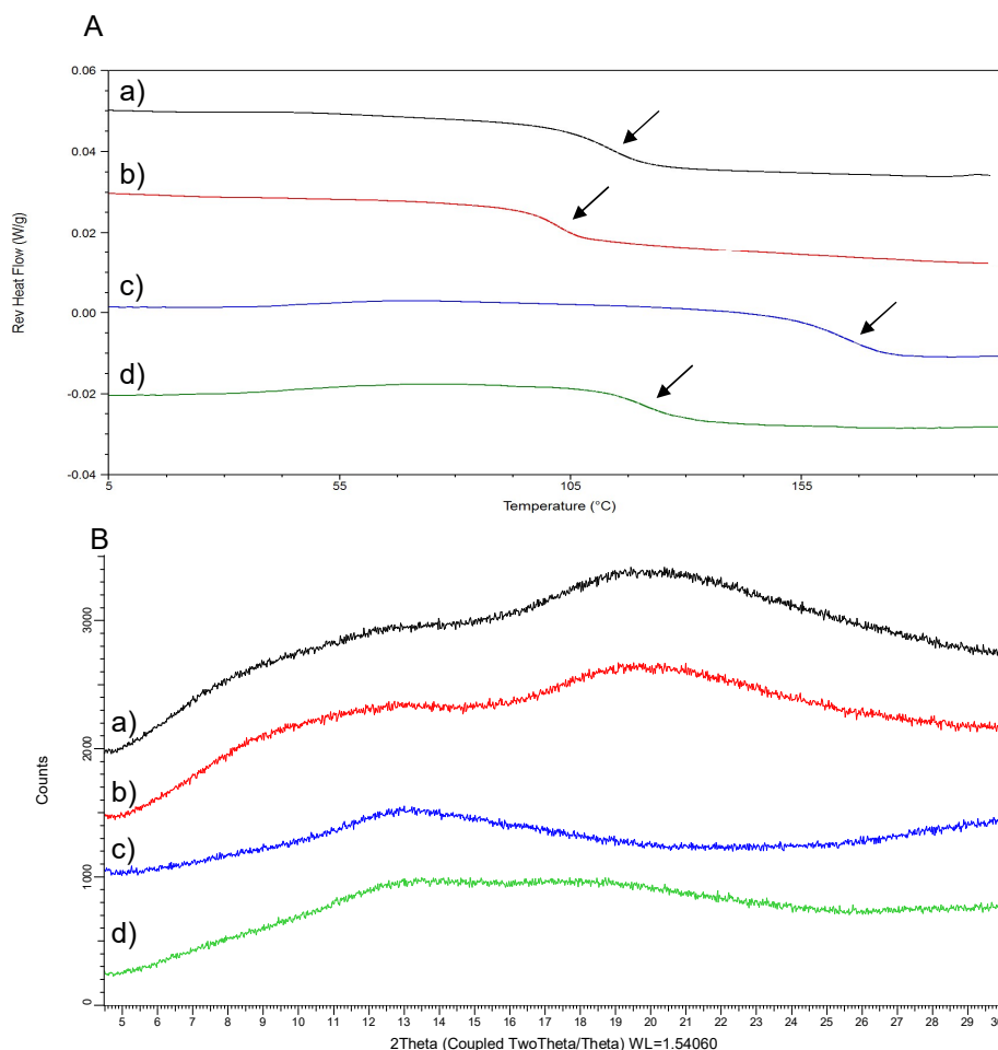
Figure 4. Reverse heat flow signals (A) and X-ray powder diffraction (XRPD) patterns (B) of 40:60 ( w/w ) CDP146 SDDSs (20 mg) made with HPMCP HP50 (a), HPMCAS-LF (b), Eudragit L100 (c) and Eudragit L100-55 (d).
