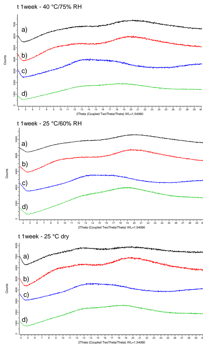
Figure 5. XRPD patterns of 40:60 ( w/w ) CDP146 SDSs (100 mg) made with HPMCP HP50 (a), HPMCAS-LF (b), Eudragit L100 (c) and Eudragit L100-55 (d) after 1 week under stress and standard storage conditions.
