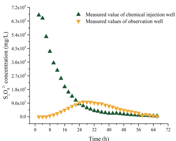
Fig. 11 S_2O_8^{2-} concentrations between days 0 and 68.
