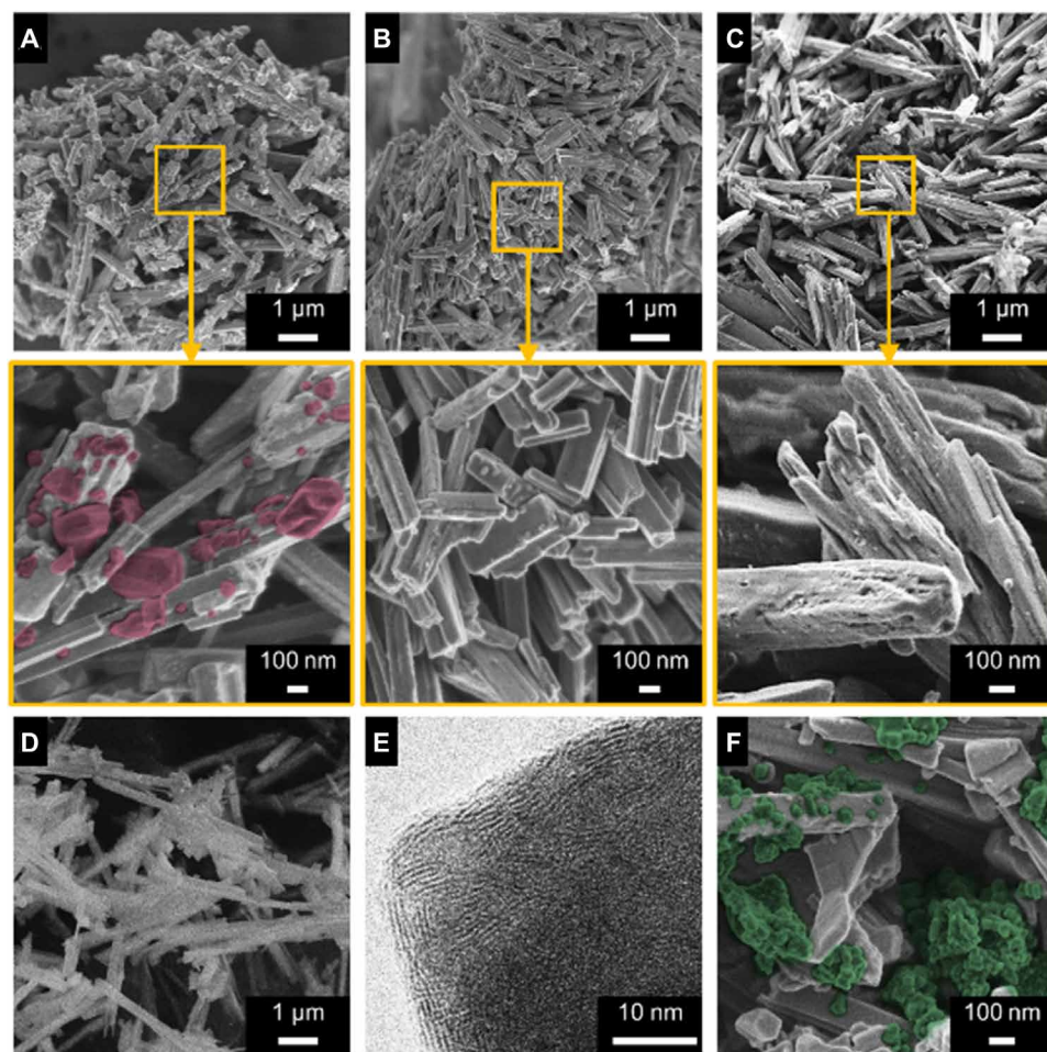
Fig. 1. Electron micrographs. (A) SEM of NiMo-3 before leaching with enlarged view below showing \text{MoS}_2 rods and compact \text{NiS}_x particles in false color. (B) SEM of NiMo-3 after leaching showing only \text{MoS}_2 rods. (C) SEM of NiMo-1 after leaching with enlarged view below showing corrugated surface of \text{MoS}_2 rods. (D) \text{MoO}_3 catalyst precursor used in hydrothermal synthesis. (E) Transmission electron micrograph of sulfided NiMo-3 after acid treatment. (F) SEM showing agglomerates of unidentified fine particles on NiMo-4 before leaching.
