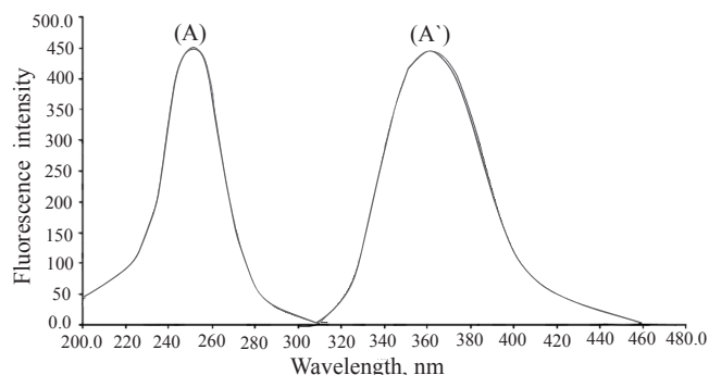
Figure 2. Excitation and emission spectra of induced Ce(III) by oxidation of 0.06 \mu\text{g mL}^{-1} DLT with Ce (IV) where: (A), Excitation spectrum; (A'), Emission spectrum.
