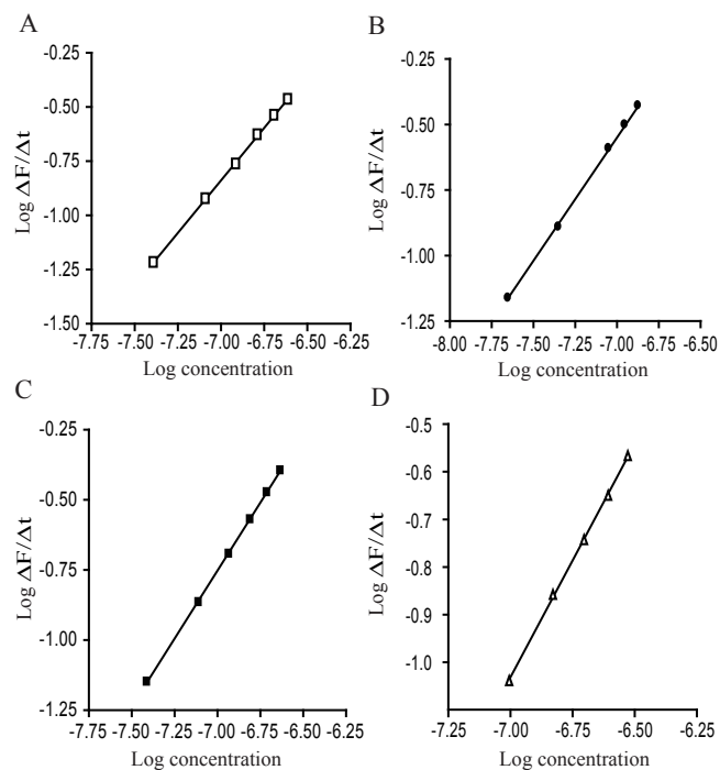
Figure 6. Plot of Log reaction rate ( \text{Log } \Delta F/\Delta t ) versus Log concentration of: A, VP; B, DLT; C, NC; D, FZ.
