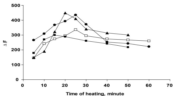
Figure 5. Effect of the heating time on the relative fluorescence intensity. \Delta , 0.06 \mu\text{g mL}^{-1} DLT; \bullet , 0.1 \mu\text{g mL}^{-1} VP; \square , 0.1 \mu\text{g mL}^{-1} FZ; \blacksquare , 0.1 \mu\text{g mL}^{-1} NC.
