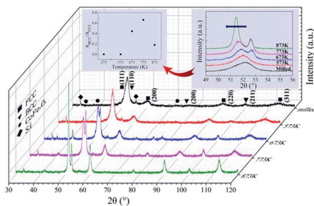
Fig. 8 XRD patterns of the as-milled and as-annealed (573–873 K) FeCoNiSi 0.3 Al 0.4 alloy powders, and the inset present the detailed scans in the range of 2\theta = 49\text{--}56^\circ . The relative content of BCC to FCC ( A_{BCC}/A_{FCC} ) for different anneal temperature are also presented in the illustration.
