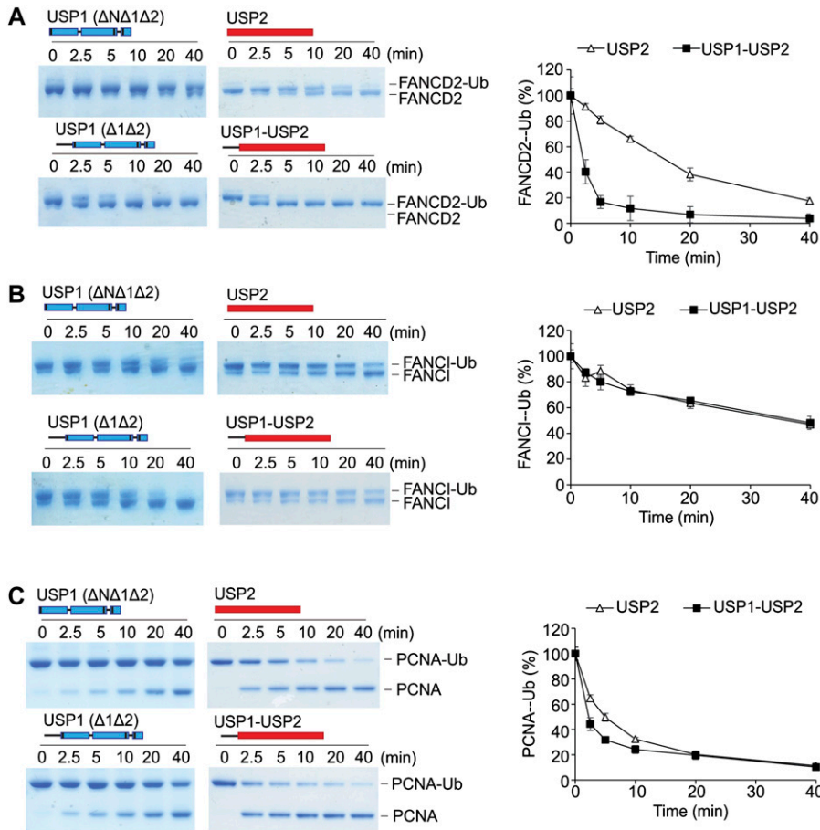
Figure 6. The N-terminus provides a gain of FANCD2-Ub activity when fused to USP2. (A) Deubiquitination of 1 \mu M FANCD2-Ub by either 100 nM of E. coli -expressed USP1 ^{\Delta N\Delta 1\Delta 2} -UAF1, USP1 ^{\Delta N\Delta 1\Delta 2} -UAF1, rat USP2 catalytic domain (USP2cat), or USP1(1-60)-USP2cat chimera, where residues 1-60 of USP1 are fused to the N-terminus of USP2's catalytic domain. Coomassie-stained FANCD2-Ub was scanned and intensity of the FANCD2-Ub band measured over time. Data show mean residual FANCD2-Ub signal (% of input) plotted against time (n = 3) \pm SD. (B) 1 \mu M FANCI-Ub and (C) 3 \mu M PCNA-Ub deubiquitination as above. Data show mean residual FANCI-Ub or PCNA-Ub signal (% of input) plotted against time (n = 3) \pm SD. Source data are available online for this figure.
