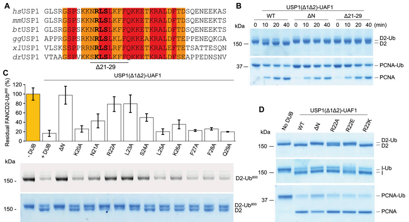
Figure 5. Several highly conserved residues within USP1 N-terminus determine FANCD2-Ub deubiquitination. (A) Sequence alignment of USP1 N-terminus from several species (hs, Homo sapiens ; mm, Mus musculus ; bt, Bos taurus ; gg, Gallus gallus ; xl, X. laevis ; dr, Danio rerio ). Deleted USP1 residues in (B) and residues important for activity (bold) in (C) are indicated. (B) Deubiquitination assay of hsFANCD2-Ub and hsPCNA-Ub using E. coli -purified USP1 Δ1Δ2 , USP1 ΔNΔ1Δ2 , and USP1 Δ21-29Δ1Δ2 in complex with UAF1. (C) Deubiquitination assays of hsFANCD2-Ub 800 by recombinant USP1 Δ1Δ2 with Ala point mutants from E. coli . The loss in fluorescence intensity was quantified and normalised to the amount of input hsFANCD2-Ub 800 . Data display mean residual FANCD2-Ub 800 (%) (n = 3) ± SD normalised to input. (D) Deubiquitination assays of hsFANCD2-Ub for 40 min using USP1 Δ1Δ2 with R22 point mutations indicate that a positive charge at position 22 is critical for hsFANCD2-Ub deubiquitination but not for hsFANCI-Ub or hsPCNA-Ub . Source data are available online for this figure.
