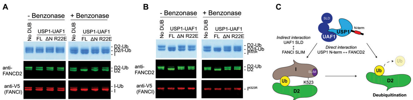
Figure 7. The N-terminus of USP1 is required for FANCD2-Ub deubiquitination when in complex with FANCI and DNA. (A) Deubiquitination of di-monoubiquitinated FANCD2-FANCI complex with and without DNA by USP1 ^{FL} -UAF1, USP1 ^{\Delta N} -UAF1, and USP1 ^{R22E} -UAF1. A FANCD2-FANCI-ds DNA complex is monoubiquitinated by Ube2Tv4, FANCL ^{\Delta E L F} , E1, and ubiquitin for 30 min and reactions arrested using apyrase. Ubiquitination reactions are treated with benzonase nuclease for 4 h on ice before being subject to USP1 for 30 min at room temperature. FANCD2 and FANCI are detected by Coomassie staining or Western blotting on the same nitrocellulose membrane and visualised using anti-FANCD2 or anti-V5 (FANCI). (B) Assay performed as in (A) except that FANCI with a K523R mutation is used. (C) Model of FANCD2-Ub deubiquitination by USP1-UAF1. USP1 targets FANCD2 via a direct interaction using its N-terminus. In addition to the N-terminus of USP1, FANCD2-Ub-FANCI complexes might be indirectly targeted by an interaction between UAF1 SLD and FANCI SUMO-like interacting motif (SLIM). Source data are available online for this figure.
