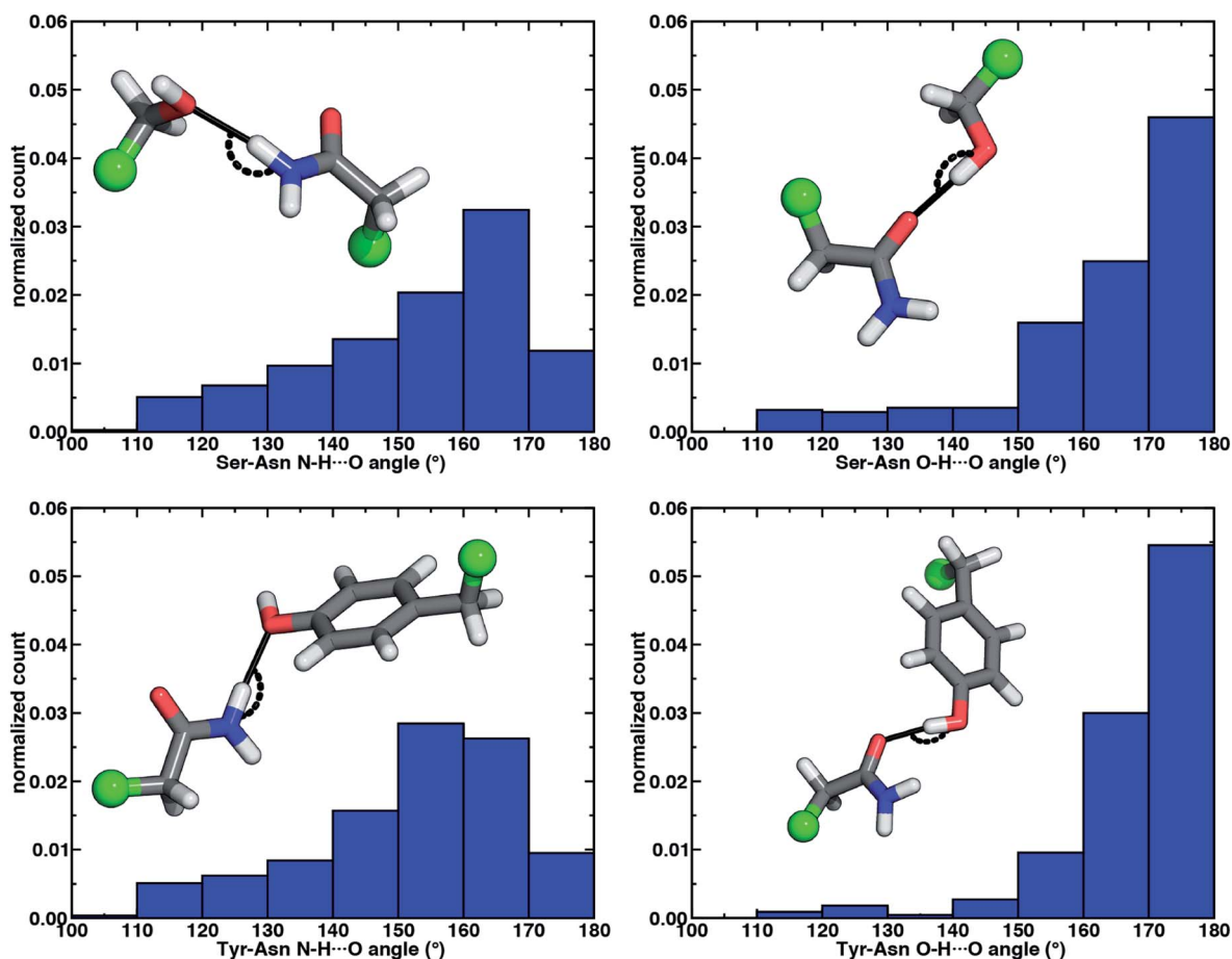
Fig. 4 Normalized histograms of N–H \cdots O HB (left) and O–H \cdots O HB (right) angles (in ^{\circ} ) for Ser–Asn (top) and Tyr–Asn (bottom) residue pairs from X-ray crystal structures. All histograms have 10^{\circ} bin widths. The structure insets depict the HB angle on representative protein structure sidechains with the corresponding C_{\alpha} of the residues represented as a green sphere and the remaining atoms shown as sticks with carbon in gray, hydrogen in white, nitrogen in blue, and oxygen in red.
