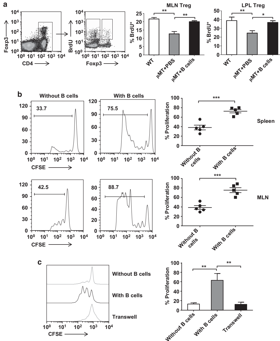
Figure 5 B cells promote regulatory T cell (Treg) proliferation. Colitis was induced as for Figure 1 in (a, b) wild-type (WT) mice and (a) \mu MT and (b) Rag^{-/-} mice that had received either phosphate-buffered saline (PBS) or 2 \times 10^7 WT splenic B cells on day -2 . (a) Bromodeoxyuridine (BrdU) was added to the drinking water on day 3 and continued for 7 days. The percentage of BrdU^+ CD4^+ Foxp3^+ Tregs was determined by flow cytometry with the gating strategy shown in the left two panels. The bar graphs show the percentage of BrdU^+ Tregs in the mesenteric lymph nodes (MLNs) and lamina propria lymphocytes (LPL) as the mean \pm s.e.m. of six mice from one experiment, and was performed three times with similar results. (b) Splenic CD4^+ CD25^+ Tregs were fluorescence-activated cell sorting (FACS) purified and labeled with carboxyfluorescein succinimidyl ester (CFSE) before intravenous (i.v.) transfer into Rag-1^{-/-} mice with or without purified splenic B220^+ B cells. On day 10, Treg proliferation was determined by dye dilution using flow cytometry (left histograms). The percentage of Tregs that had undergone proliferation in the spleen and MLNs is shown in the right scatter graphs, with each data point representing a single mouse. The data shown are the mean \pm s.e.m. from one experiment with five mice and was repeated twice with similar results. (c) Splenic Tregs ( CD4^+ CD25^+ ) were purified by FACS and cultured alone ( 2 \times 10^5 cells) or with splenic B220^+ B cells ( 2 \times 10^5 ) that were placed either in the culture well or in a transwell in the presence of anti-CD3 ( 1 \mu g ml^{-1} ) and anti-CD28 ( 5 \mu g ml^{-1} ) in the presence or absence of B cells for 72 h after which Treg proliferation was determined by CFSE dye dilution by flow cytometry. A representative histogram is shown on the left and the bar graph is the mean \pm s.e.m. of three independent experiments each with three mice. * P < 0.05 ; ** P < 0.01 ; *** P < 0.001 .
