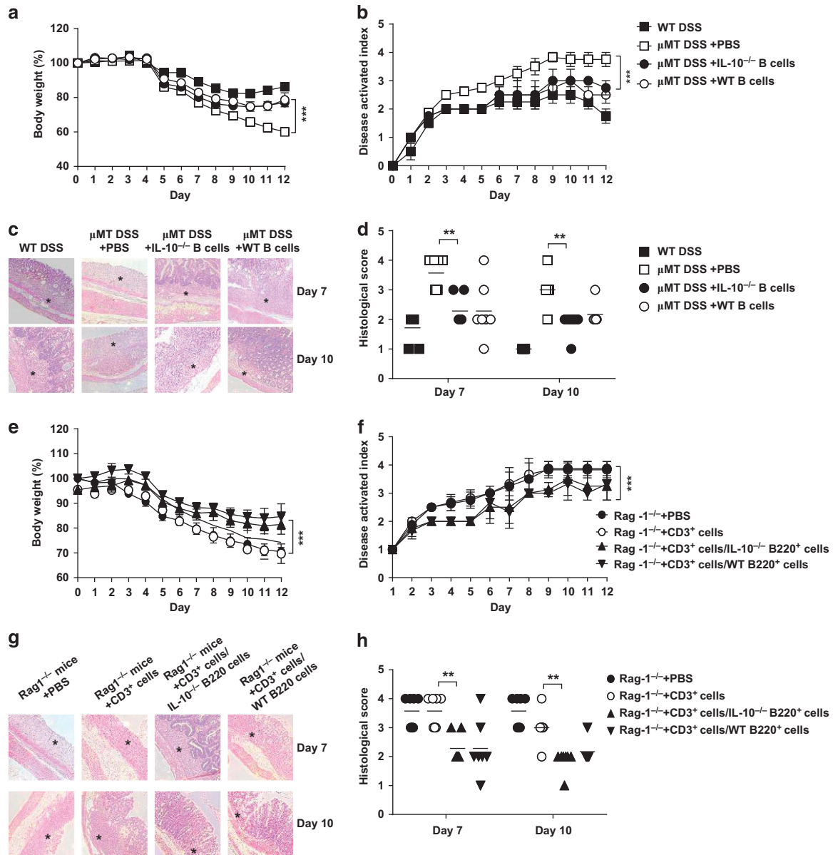
Figure 2 Attenuation of colitis by B cells does not require their production of interleukin-10 (IL-10). Colitis was induced in (a–d) wild-type (WT), (a–d) \mu MT, or (e–h) Rag1 -/- as for Figure 1. PBS, phosphate-buffered saline. (a–d) On day -2 of dextran sulfate sodium (DSS)-induced colitis, \mu MT mice were intravenously (i.v.) administered 2 \times 10^7 splenic WT or IL-10 -/- B cells (B220 + ) and (e–h) Rag1 -/- mice were similarly administered splenic CD3 + T cells or CD3 + T cells and either WT or IL-10 -/- B cells. Mice were evaluated daily for (a, e) weight loss and (b, f) disease activity index (DAI) scores were calculated. Representative colon histological sections stained with hematoxylin and eosin (H&E) are shown for the (c) WT and \mu MT and (g) Rag1 -/- groups of mice at days 7 and 10 after colitis induction. Images are shown at original magnification \times 200 . An asterisk indicates the position of the leukocyte infiltration in the histological images. (d, h) Histological sections were scored as for Figure 1 with each data point representing a single mouse. (a, b, e, f) The data shown are the mean \pm s.e.m. from one experiment with seven mice and was repeated three times with similar results. ** P < 0.01 ; *** P < 0.001 ).
