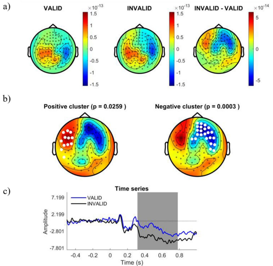
Figure 3. Represents the distribution of cortical activity from 310 to 780 ms. (a) Shows topographical maps of amplitudes for each condition (left and central map) and their arithmetic subtraction (right map). (b) Represents statistical differences (T values) between conditions. Left, positive cluster, and right, negative cluster. White dots represent sensors that showed significant differences during time-window. (c) Shows the whole time-series for both conditions (blue = VALID; black = INVALID). Grey mask represents time-slice of samples with significant results.
