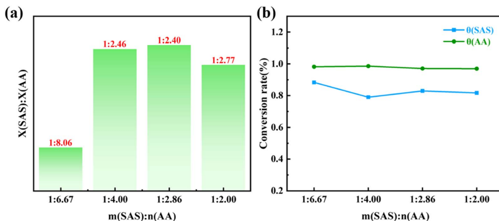
Fig. 4 (a) Histogram of feeding ratio versus structural unit composition ratio in \text{p}(\text{AA-co-SAS}) ; (b) relationship between feed ratio and monomer conversion.
