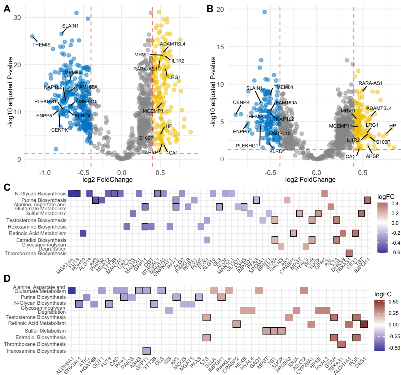
Figure 5 Correlations of the COPD subtypes with transcription features in the ECLIPSE dataset. (A) Volcano plot showing all differentially expressed genes (DEGs) with an RRA score <math>< 0.05</math> between two subtypes in the ECLIPSE dataset. The top 10 upregulated and downregulated genes ranked by RRA score are labelled in the figure. (B) Volcano plot showing all differentially expressed genes with an RRA score <math>< 0.05</math> between the two subtypes in the COPDGene dataset. (C) Heatmap displaying DEGs from 10 metabolic pathways in the ECLIPSE dataset. (D) Heatmap displaying DEGs from 10 metabolic pathways in the COPDGene dataset. The genes with overlapping of two datasets are highlighted by black border.
