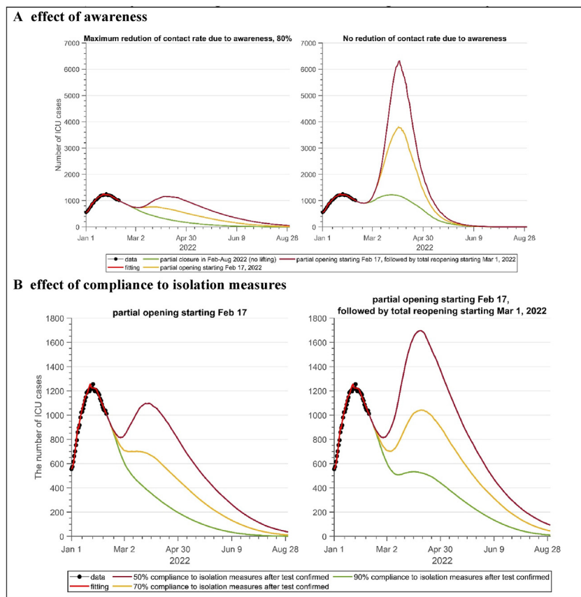
Fig. 7. The impact of social behaviors on the daily ICU occupancy in Canada after lifting the restriction measures.
