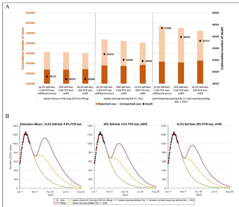
Fig. 5. Simulation results for Canada as a whole under scenarios for testing strategies & lifting of restrictions. Panel A: the cumulative case count & death in Canada up to August 31, 2022; Panel B the epidemic curves for the scenarios.
