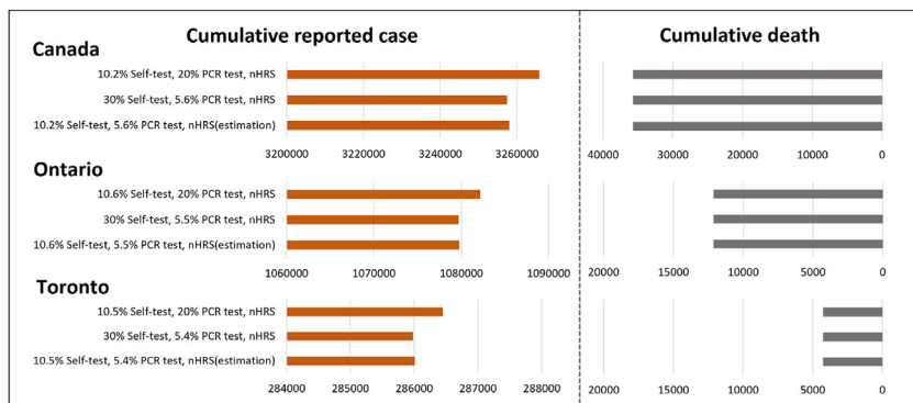
Fig. 4. The impact of different test strategies on the COVID cases and death in Toronto, Ontario, and Canada, in the short run. The cumulative number of cases and death are the projections till February 15, 2022 (the 2 incubation periods after data).
