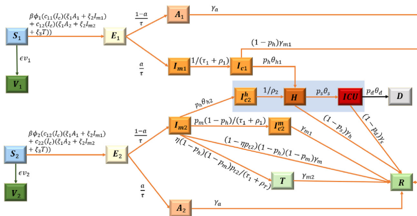
Fig. 1. Diagram for the transmission in high-risk settings (subscript 1) and non high-risk settings (subscript 2).
