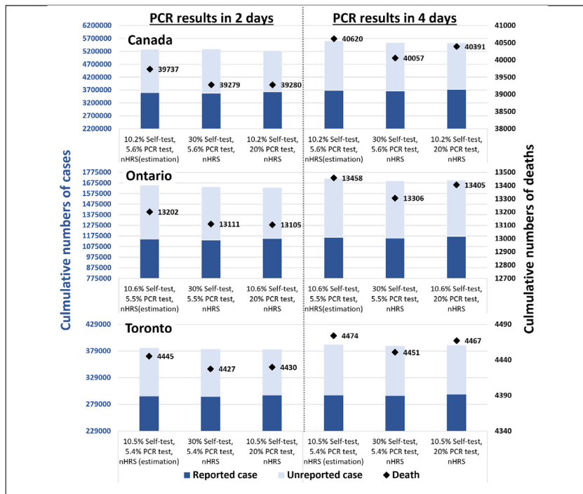
Fig. 3. The impact of increasing PCR result turnaround time to 2 days (left hand column) from 4 days (right hand column). The cumulative number of cases and death are the projections till Aug 31, 2022 (scenario B in Table 1).
