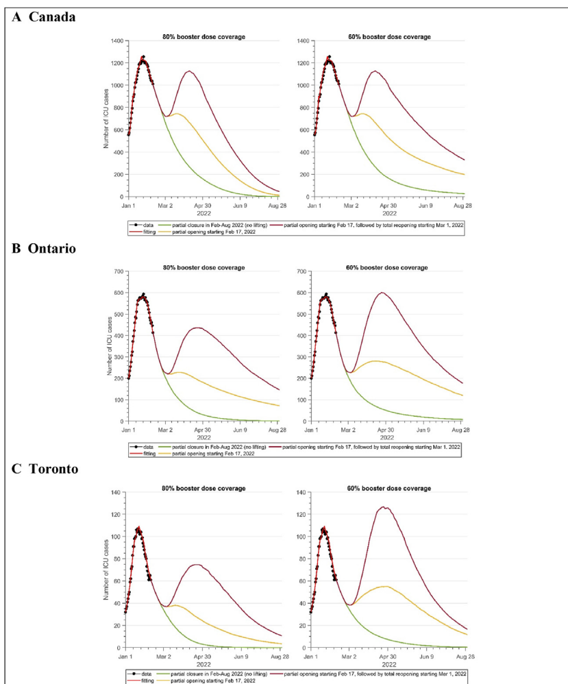
Fig. 6. The impact of booster dose coverage on the daily ICU occupancy after lifting the restriction measures. (A) Canada (B) Ontario (C) Toronto.
