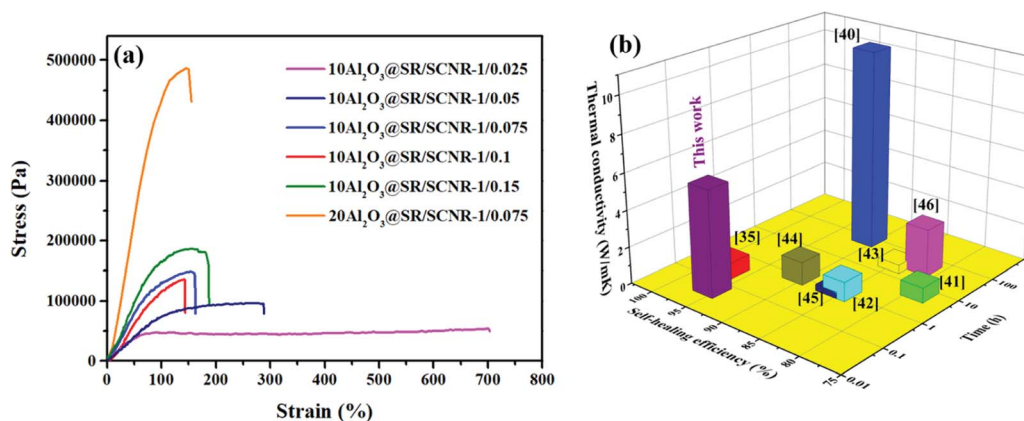
Fig. 7 (a): Stress–strain curve of \text{Al}_2\text{O}_3@SR/SCNR composites; (b) the comparison of time on healing, thermal conductivity and self-healing efficiency between 20\text{Al}_2\text{O}_3@SR/SCNR-1/0.075 and previously reported works.
