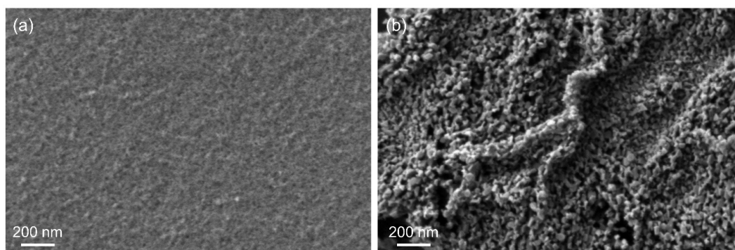
Figure 4. SEM images of two example layers of (a) Al 2 O 3 and (b) MgO prepared by pre-mixing the polymer ((a): 200 mg; (b): 150 mg) with the metal salts ((a): 600 mg Al(NO 3 ) 3 ·9H 2 O; (b): 450 mg Mg(NO 3 ) 2 ·6H 2 O) prior to spin-coating and subsequent photo-cross-linking and calcination.
