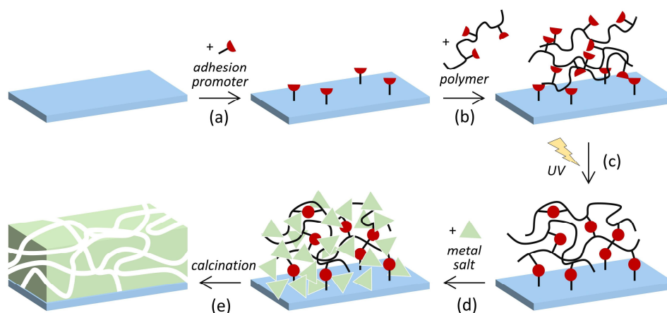
Scheme 1. Preparation of porous metal oxide ( \text{Al}_2\text{O}_3 , MgO) layers: (a) anchoring of the adhesion promoter on the Si wafer substrate; (b) spreading of the polymer by spin coating; (c) hydrogel formation and immobilization on the substrate by photo-induced cross-linking; (d) swelling in metal salt solution ( \text{Al}(\text{NO}_3)_3 , \text{Mg}(\text{NO}_3)_2 ); (e) formation of the porous metal oxide and combustion of the hydrogel by calcination.
