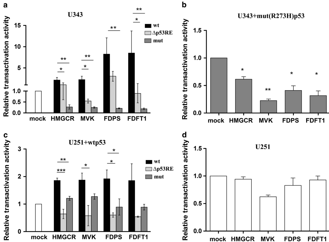
Figure 4 Luciferase reporter assays in glioblastoma cells. (a) U343 cells were transiently transfected with three different pGL3 plasmids wt: containing the promoter regions containing p53RE (wild type) from HMGCR, MVK, FDPS and FDFT1 gene sequences, Δp53RE: the constructs with deleted-cloned sequences of the mentioned genes (Δp53RE) and mut: the constructs containing promoter regions with single mutation of p53 of HMGCR, MVK, FDPS and FDFT1 genes (mut). (b) U343 cells were co-transfected with mut (R273H) p53 plasmid and with constructs containing promoter regions. (c) wt p53-transfected U251 cells were co-transfected with constructs containing wt and mutated promoter regions of enzymes of MVA pathway. (d) U251 cells were transfected with promoter regions–constructs of MVA enzymes. Results were normalized for β-galactosidase activity and compared with results obtained in cells transfected with empty vector (mock). Data represent mean ± S.D. of three independent experiments and statistical analysis was performed with one-way ANOVA, * P \leq 0.05 ; ** P \leq 0.01 ; *** P \leq 0.001
