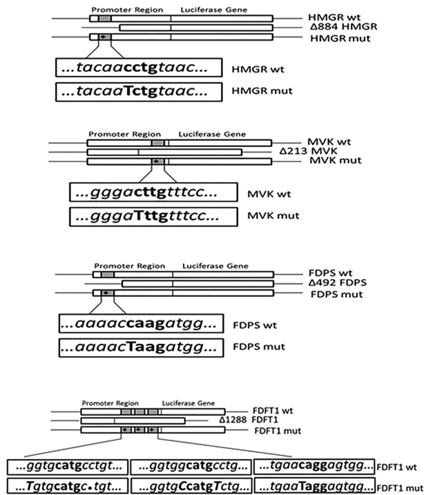
Scheme 2 Promoter regions containing p53REs cloned in pGL3 luciferase reporter vector. p53REs positive to ChIP assays were cloned and integrated in a pGL3 luciferase reporter vector to evaluate the link between these potential promoter regions and p53 transcriptional activity. Regions cloned from HMGR, MVK, FDPS, FDFT1 genes were also deleted and mutated in p53RE and subsequently tested for luciferase transcription ability
