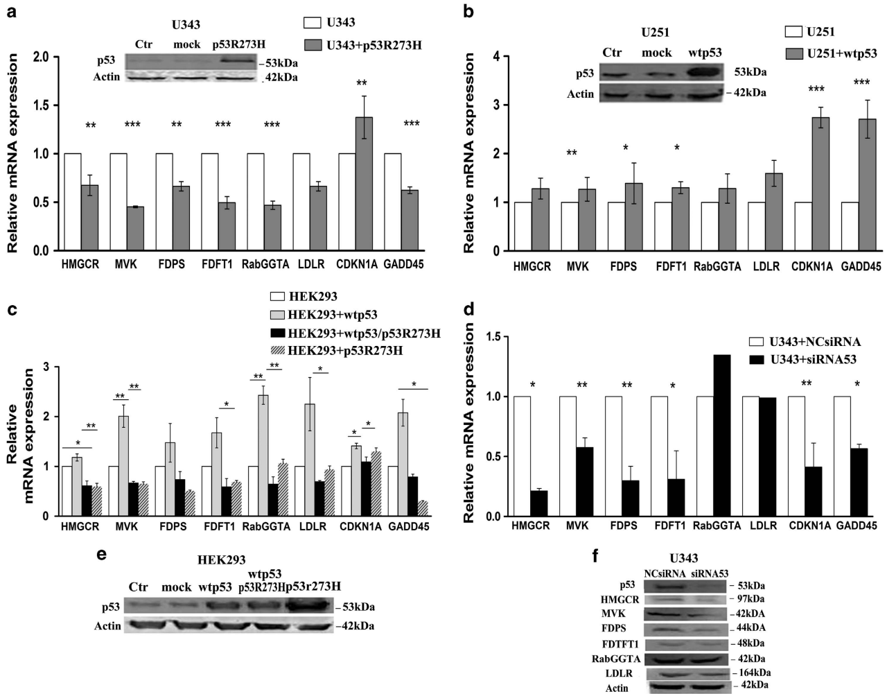
Figure 2 Analysis of mRNA levels of enzymes related to MVA pathway upon genetic perturbation of p53. qRT-PCR analysis of MVA pathway enzymes in (a) U343 cells untransfected and transfected with empty vector control (mock) or with mutant (R273H) p53. Data were analyzed with a two-tailed t -test. Western blot showed p53 protein levels following transfections with the plasmid constructs in U343 cells (ctr = untransfected cells; mock = cells transfected with empty vector; U343+p53(R273H) = cells transfected with mutant p53). (b) U251 cells transfected with empty vector control or with vector containing wild-type p53 (pCMVp53). Western blot shows p53 protein levels following transfections. (c) HEK293 cells transfected with control empty vector (mock), or with pCMVp53 alone, co-transfected with construct containing with mutant p53 or transfected with (R273H) p53 alone. Western blot shows the transfection efficiency. Data are mean \pm S.D. of three independent experiments. One-way ANOVA analysis indicated a significant difference in genes expression (** P \leq 0.001 ; * P \leq 0.05 ). (d) Knockdown of wt p53 from U343 cell line: cells transfected with siRNA p53 downregulated the expression and the protein levels of enzymes of MVA pathway (f). A representative actin was used for all samples as loading control. (e) Western blot analyses shows the overexpression of p53 after transfection in HEK293 cell line in the several experimental conditions. *** P \leq 0.001
