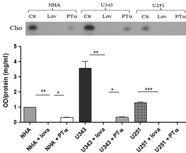
Figure 7 [ 14 C]-acetate incorporation in neo-synthesized CHO. Chromatogram of non-saponifiable lipids from cells radiolabeled during a 14-h period following treatment. U343 and U251 cells were incubated with Lov (10 μM for 24 h) and cyclic PT-α (30 μM for 24 h). CHO bands are indicated with an arrow and the graphic represents densitometric analysis of two independent experiments. Statistical analysis was performed with one-way ANOVA * P ≤ 0.05; ** P ≤ 0.01; *** P ≤ 0.001
