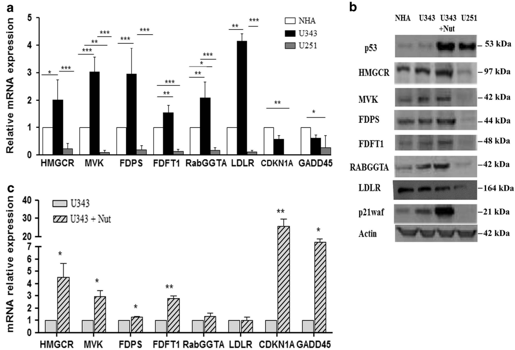
Figure 1 HMGR, MVK, FDPS, FDFT1, RabGGTA and LDLR expression in different cell lines. (a) qRT-PCR analyses in U343 cells with wild-type p53, U251 cells bearing a mutant p53 (R273H) and NHA cells used as reference cell line for basal levels. CDKN1A and GADD45 genes served as a positive control. All the data represented mean \pm S.D. of five independent experiments. Statistical analysis was conducted with one-way ANOVA and columns indicated with asterisks represent a significant difference in gene expression levels ( ***P \leq 0.001 ; **P \leq 0.01 ; *P \leq 0.05 ) compared with NHA control cells. (b) Western blot analyses of protein levels of the MVA pathway enzymes and p21waf. A representative actin was used for all samples as control. (c) qRT-PCR analysis of MVA pathway enzymes was conducted for U343 cells treated or not with Nut at 10 \mu\text{M} for 24 h. Data are representative of three different experiments. A two-tailed t -test was conducted as statistical analysis. Columns indicated with asterisks represent significant increase compared with unmarked columns ( **P \leq 0.01 ; *P \leq 0.05 )
