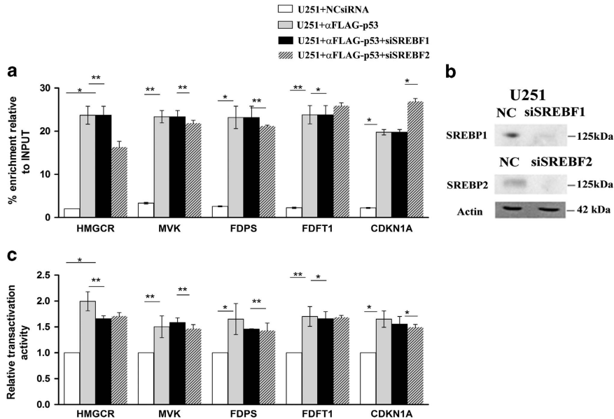
Figure 6 (a) ChIP assays and (c) Luciferase reporter analysis of U251 cells after knockdown of SREBP1 and SREBP2. U251 cells were co-transfected with FLAG-p53 and control siRNA or siRNA directed against SREBP1 and SREBP2. (b) Immunoblot shows knockdown of SREBP1 and SREBP2. Actin was made as control of loading. Data represent mean \pm S.D. of three independent experiments and statistical analysis was performed with one-way ANOVA, * P \leq 0.05 ; ** P \leq 0.01
