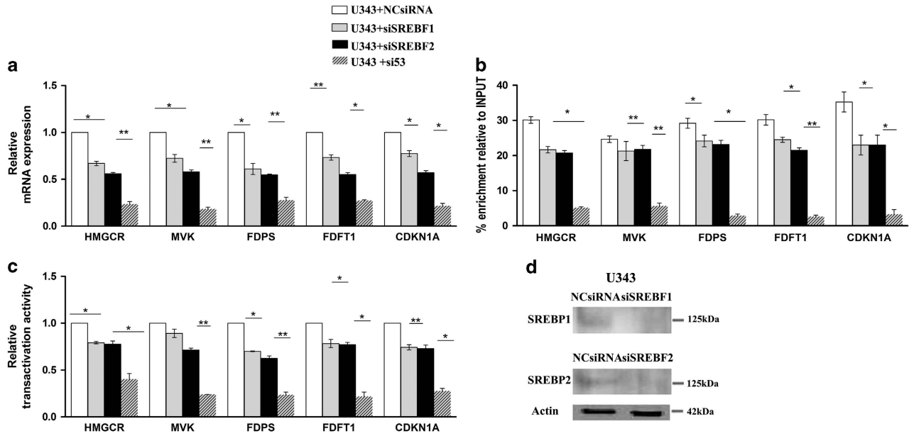
Figure 5 (a) qRT-PCR of enzymes related to MVA pathway, (b) ChIP assays and (c) luciferase reporter analysis of U343 cells after knockdown of SREBP1, SREBP2 and p53. U343 cells were treated with a control siRNA or siRNA directed against SREBP1, SREBP2 and p53. (d) Immunoblot shows knockdown of SREBP1 and SREBP2 (see also Figure 3f for the depletion of p53). Actin was made as control of loading. Data represent mean \pm S.D. of three independent experiments and statistical analysis was performed with one-way ANOVA, * P \leq 0.05 ; ** P \leq 0.01
