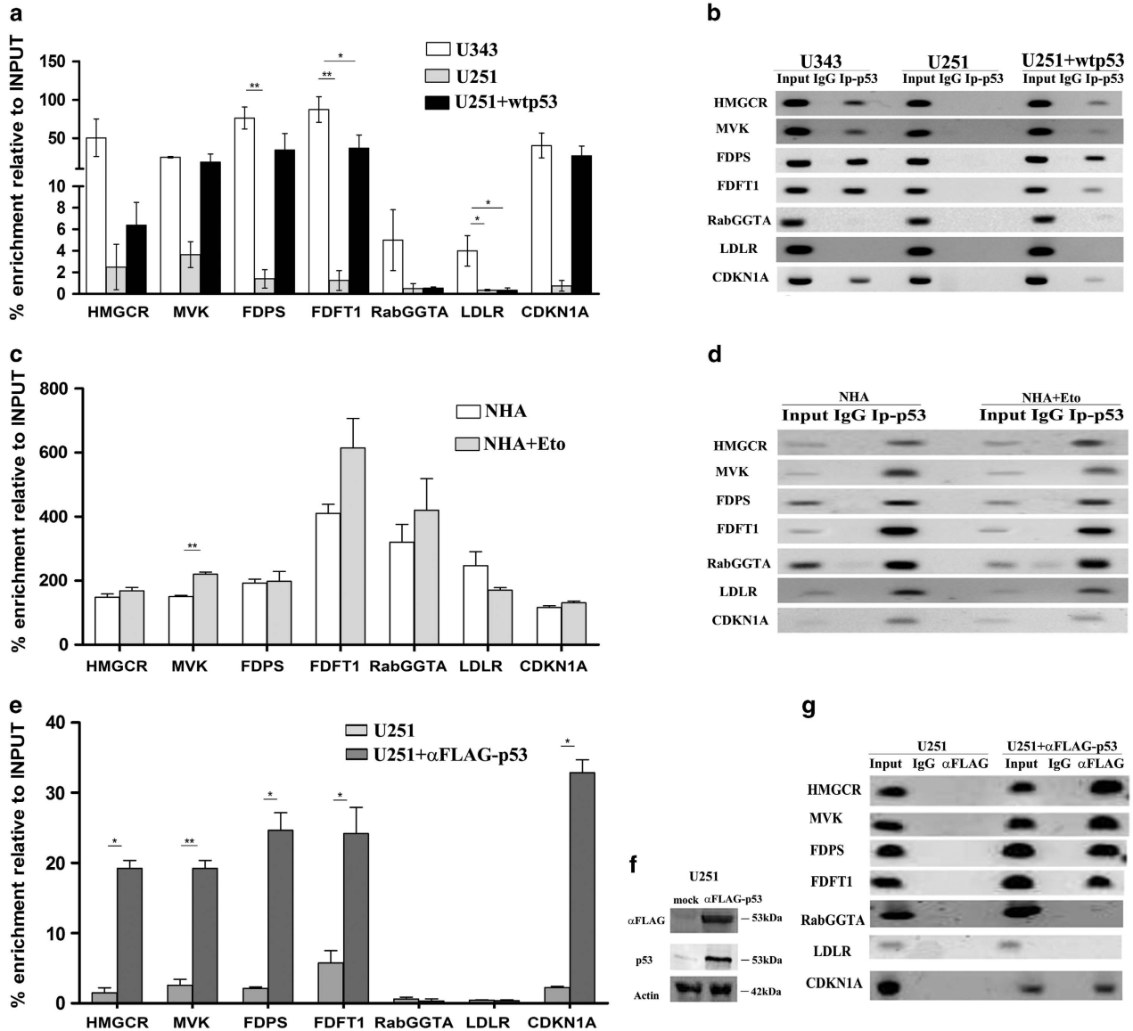
Figure 3 ChIP assays in glioblastoma cells. Chromatin samples from (a) U343 cells, U251 cells and pCMVp53 transfected U251 cells were immunoprecipitated in the presence of control rabbit IgG or with specific antibody anti-p53. p53 is immunoprecipitated along with p53REs of promoter of HMGR, MVK, FDPS, FDFT1. qRT-PCR analysis was conducted using primers set specific for putative p53REs (Supplementary table 3). Obtained results were normalized to 1% input. (b) Representative agarose gels of PCR products of ChIP assay using an antibody against p53 and anti-rabbit IgG as control of U343 cells, U251 cells and U251 transfected with p53wt. (c) qRT-PCR analysis of p53REs co-immunoprecipitated with p53 in NHA cells untreated and treated with eto at 25 \mu M for 24 h. All the data are reported as mean \pm S.D. of two independent experiments. One-way ANOVA was performed to indicate significant differences in genes expression. CDKN1A promoter was used as a positive control. (d) Representative agarose gels of PCR products of ChIP assay using an antibody against p53 and anti-rabbit IgG as control of NHA and NHA treated with eto. (e) Chromatin samples from U251 transfected with FLAG-p53 or with an equivalent amount of empty vector were immunoprecipitated with anti-mouse IgG, anti-FLAG or p53 antibodies as indicated. qRT-PCR analysis was conducted using primers set specific for putative p53REs. (f) Western blot reports the amounts of FLAG-p53 and of p53 in one typical experiment. Actin was made as control of loading. (g) Representative agarose of PCR products of ChIP assay using an antibody against FLAG and anti-rabbit IgG as control of U251 cells transfected with FLAG-p53 and equivalent amount of empty vector. One-way ANOVA analysis indicated a significant difference in genes expression (* P \leq 0.05 ; ** P \leq 0.001 )
