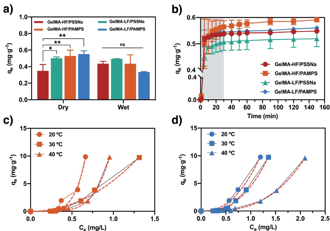
Fig. 5 Adsorption of MB by the GelMA composite hydrogel: (a) comparison of the dry and wet hydrogel sorption behaviors ([MB] = 3.0 mg L -1 , pH = 7.4, 20 °C, 100 rpm, n = 3 ), (b) sorption kinetics, where the dashed lines corresponds to the pseudo-second order fit ([MB] = 3.0 mg L -1 , pH = 7.4, 20 °C, 100 rpm), (c) sorption isotherms of GelMA-HF/PAMPS, and (d) sorption isotherms of GelMA-LF/PAMPS, where the dashed lines correspond to the Freundlich isotherm model fit (pH = 7.4, 20 °C, 100 rpm).
