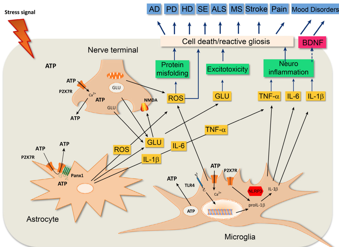
Fig. 3 Common disease mechanism by P2X7 receptor (P2X7R)-mediated pathways in central nervous system (CNS) disorders of different etiology. P2X7R are expressed on nerve terminals, astrocytes and microglia, and they are upregulated in various disease conditions. Stress signals such as hypoxia/ischemia (metabolic limitations), mechanical injury and bacterial or chemical toxins elicit the endogenous activation of P2X7R and lead to a self-amplifying ATP release and to further activation of P2X7R on neighbouring cells. Following the influx of \text{Ca}^{2+} through the receptor ion channel complex, P2X7R activation (i) releases glutamate from nerve terminals and astrocytes by both exocytotic and non-exocytotic mechanisms, which may give rise excitotoxicity; (ii) leads to the posttranslational processing of pro-interleukin-1 \beta (pro-IL-1 \beta ) to the leaderless, mature IL-1 \beta and to its further release by the NLRP3 inflammasome and that
