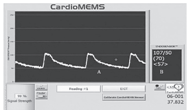
Figure 2 – Pressure wave and levels measured by the sensor during Reading 1. A. Pressure wave within the aneurysm sac. B. Various pressure levels within the sac. From top to bottom: systolic/diastolic, mean, and pulse pressure.
