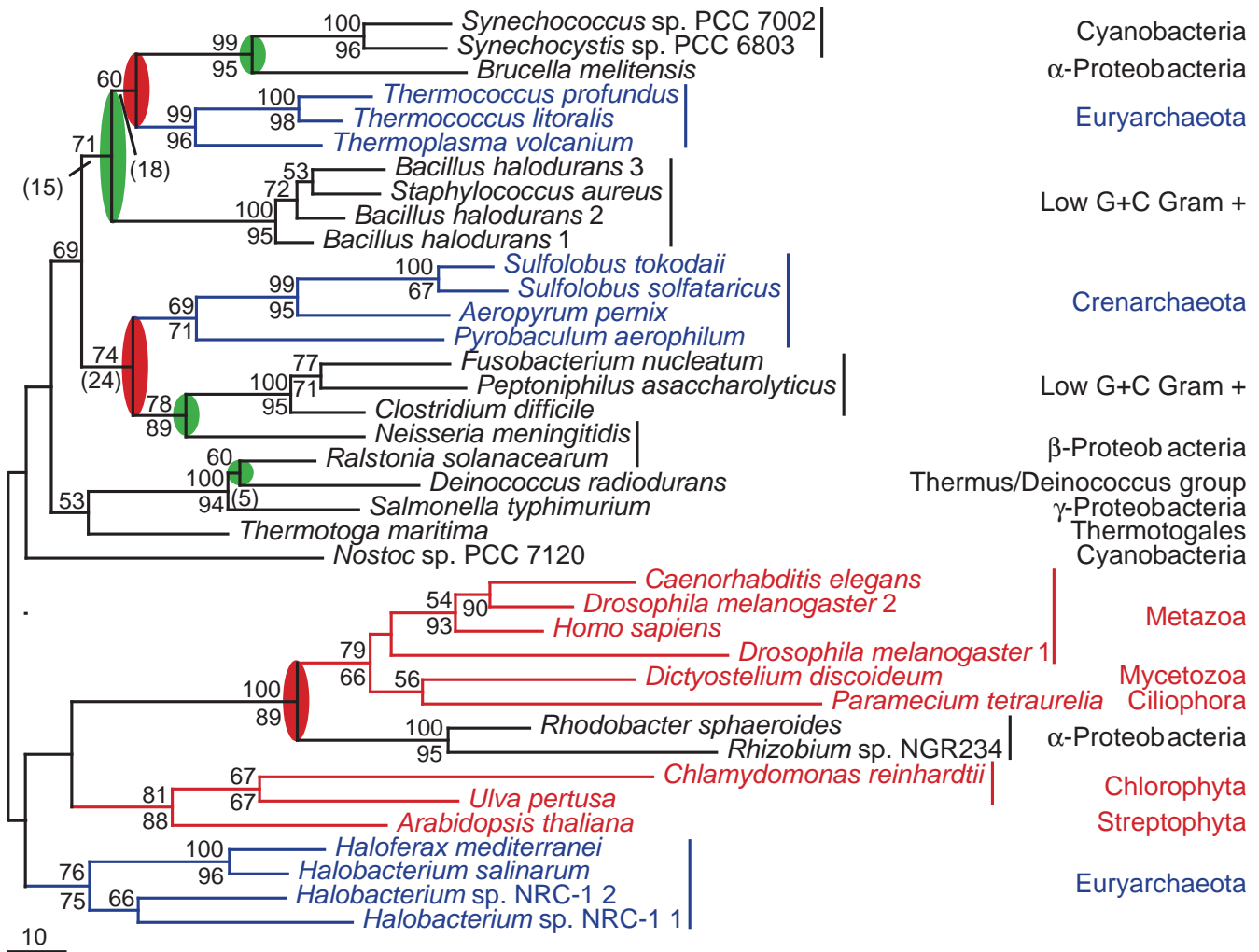
Figure 2 Maximum likelihood tree of GDH-2 The phylogenetic tree is based on 305 unambiguously aligned amino acid positions. The \Gamma shape parameter, \alpha , and the fraction of invariable sites, P_{inv} , were estimated to 1.10 and 0.08, respectively. The tree is arbitrarily rooted. Labeling as in Figure 1 with the addition that Archaea are labeled in blue.
