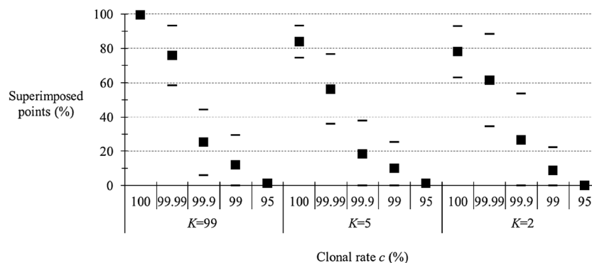
Figure 3 Proportion of superimposed points (in percent) between expected and observed F_{IS} for different levels (percent) of clonality (c) for different degrees of homoplasmy: low ( K = 99 ), medium ( K = 5 ) and maximum ( K = 2 ) in an island model with u = 10^{-5} and m = 0.01 .
