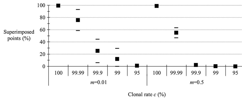
Figure 2 Proportion of superimposed points (in percent) between expected and observed F_{IS} for different levels (percent) of clonality (c), for different migration rates (m) in an island model with K = 99 and u = 10^{-5} .
