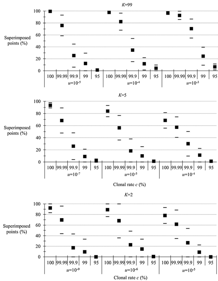
Figure 4 Proportion of superimposed points (in percent) between expected and observed F_{IS} for different levels (percent) of clonality (c) for different mutation rates (u) and different degrees of homoplasy ( K = 99 , K = 5 , K = 2 ) in an island model of migration.
