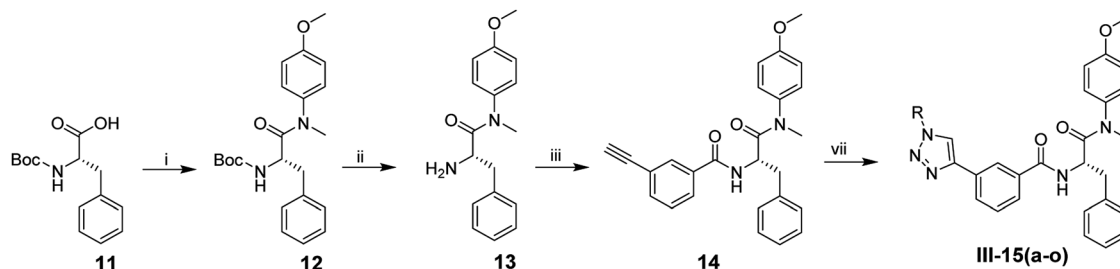
Scheme 3 Reagents and conditions used to synthesize III-15(a-o) . (i) 4-methoxy- N -methylaniline, PyBop, DIEA, CH 2 Cl 2 , r.t., 8–10 h; (ii) CF 3 COOH; CH 2 Cl 2 , r.t., 5–6 h; (iii) 3-ethynylbenzoic acid, HATU, DIEA, CH 2 Cl 2 , r.t., 10 h; (vii) azide substituents; CuSO 4 ·5H 2 O, VcNa, THF/H 2 O ( v : v = 1 : 1), 30–60 °C, 4–6 h.
