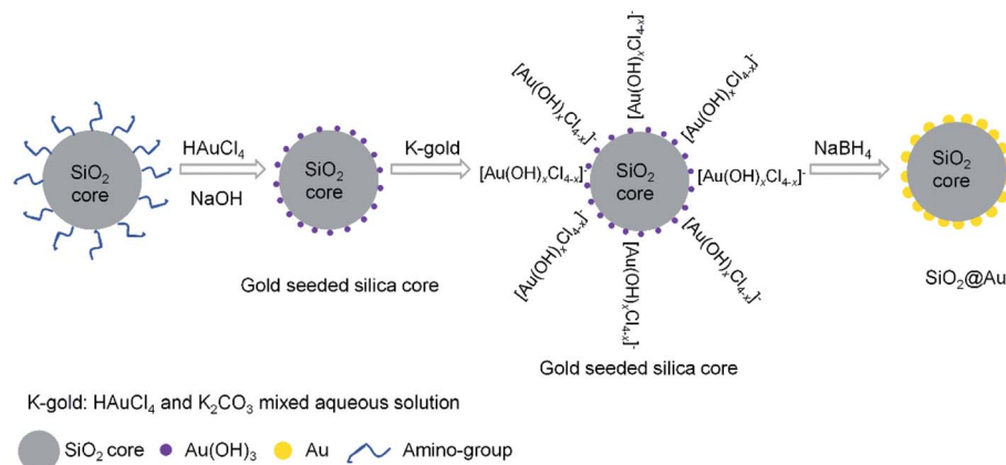
Scheme 1 Synthetic procedures of the \text{SiO}_2@Au core-shell nanoparticles.
