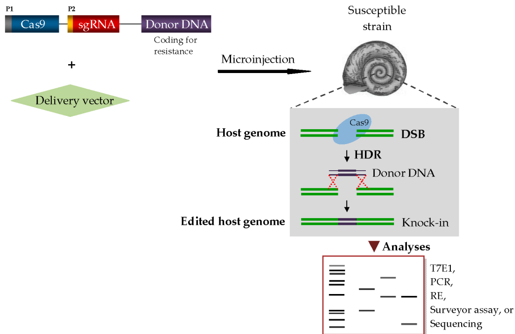
Figure 2. A schematic representation of CRISPR/Cas9 genome editing system in a snail vector of schistosome. Abbreviations: DSB, double-strand break; HDR, homology-directed repair; P1 & P2, promoters; PCR, polymerase chain reaction; RE, restriction enzyme; T7E1, T7 endonuclease I.
