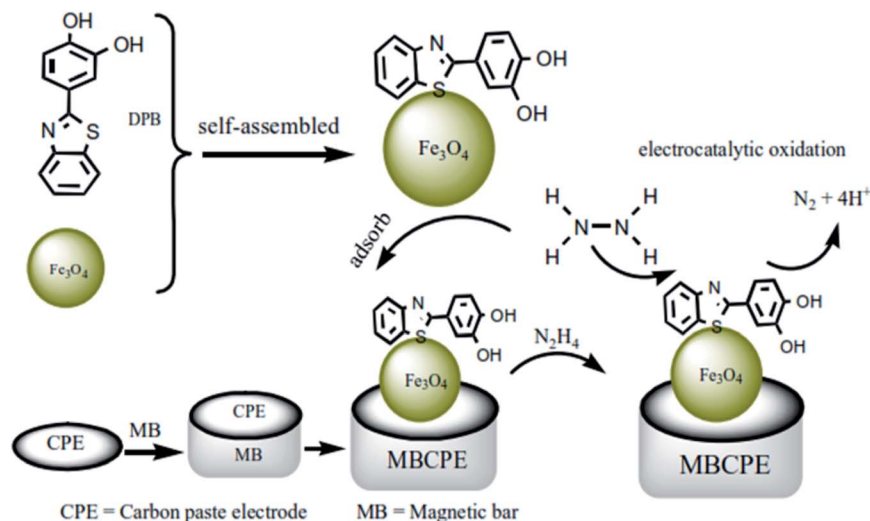
Fig. 2 Diagram of the electro-chemical detection of the HZ based on the MBCPE/ \text{Fe}_3\text{O}_4 NPs/DPB electrode. Reused with permission from ref. 58. Copyright (2016) Elsevier.
