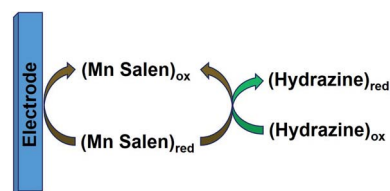
Fig. 3 The HZ electro-catalytic oxidation at the Mn(III) salen/ \text{TiO}_2 NPs/CPE.
