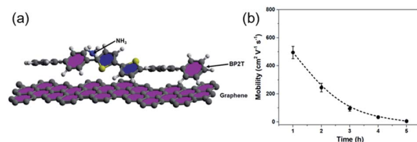
Fig. 6 (a) DFT calculation model that is used for the calculation of the absorption. (b) Plot of the measured carrier mobility as a function of immersion time.
