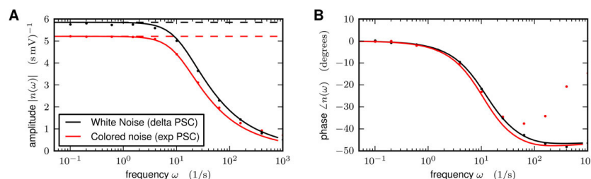
Figure 1 A Linear response amplitude for neurons exposed to colored (red) and white (black) noise. Simulations (dots) and analytical results (curves). B Phase shift of linear response.
