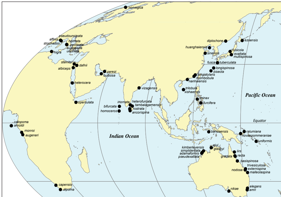
Figure 1. Hydroides species type localities of the Eastern Hemisphere (Indian Ocean and Western Pacific). Labels are current species-group names (except homonym H. rostrata renamed herein as H. gottfriedi nom. n.)
