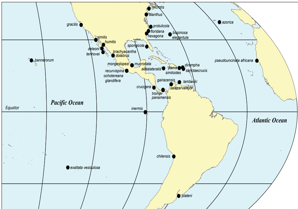
Figure 2. Hydroides species type localities of the Western Hemisphere (Americas and Eastern Pacific). Labels are current species-group names. Map grids 30° intervals.
