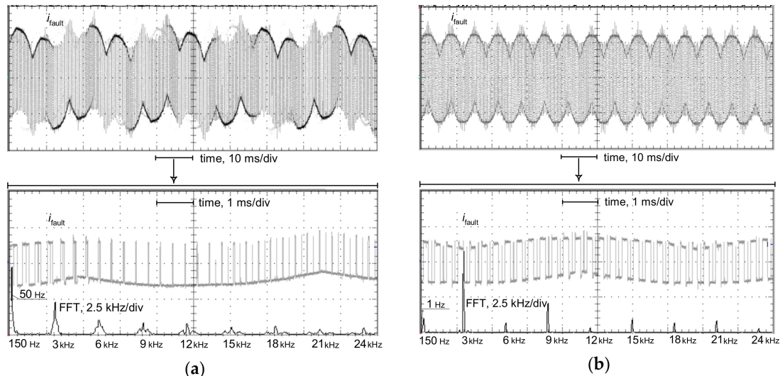
Figure 13. Oscillograms of the line-to-earth fault current waveform i_{fault} and its FFT analysis in the case of an earth fault at the output terminals of the frequency converter supplying a motor: (a) operating frequency of 50 Hz (nominal motor speed); (b) operating frequency of 1 Hz (very low motor speed); pulse width modulation (PWM) frequency of 3 kHz; line-to-earth connection via resistance of 1 k \Omega (conventional human body resistance).
