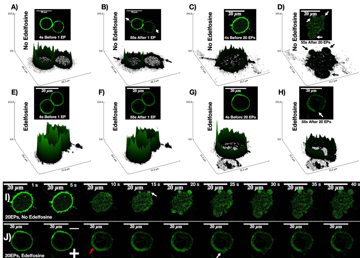
Fig. 3. Effect of PLC blockage on nsPEF induced PIP_2 cellular effects. nsPEF exposures resulted in PIP_2 depletion, as tracked by PLC6-PH-EGFP probe translocation, and cellular blebbing (A, B, C, D). 20 \mu M edelfosine pretreatment prevented all these effects after a single, 16.2 kV/cm, 600 ns EP (E and F). Twenty pulses resulted in partial PIP_2 depletion on the cell side facing the anodic electrode, with single bleb formation in the same location (G and H). Time lapse of post- 20 pulses of 16.2 kV/cm nsPEF exposure shows cellular effects in normal (I) and edelfosine-treated (J) cells.
