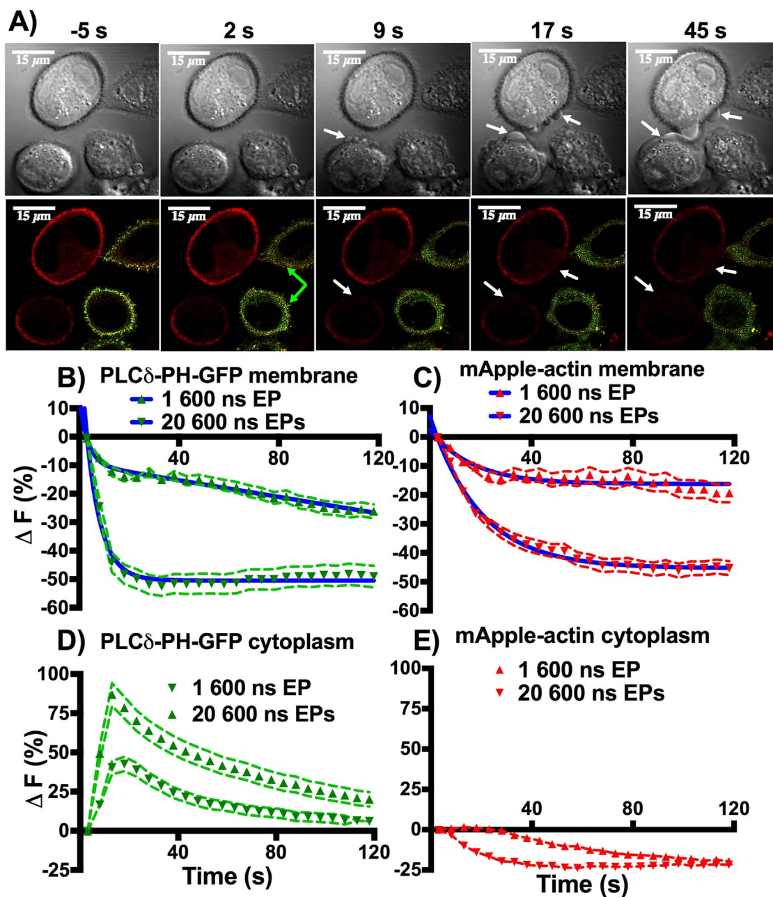
Fig. 4. Actin cortex and PIP_2 changes after nsPEF exposure. Actin cortex dissociation is directly related to PIP_2 depletion and cellular blebbing (A). Rapid PLC \delta -PH-EGFP probe translocation is observed after nsPEF exposure (B and D). A slower decrease in mApple-actin cortex fluorescence is also observed after nsPEF exposure (C), but without accumulation in the cytoplasm (E). Data are presented as mean of \Delta\% fluorescence changes with SEM.
