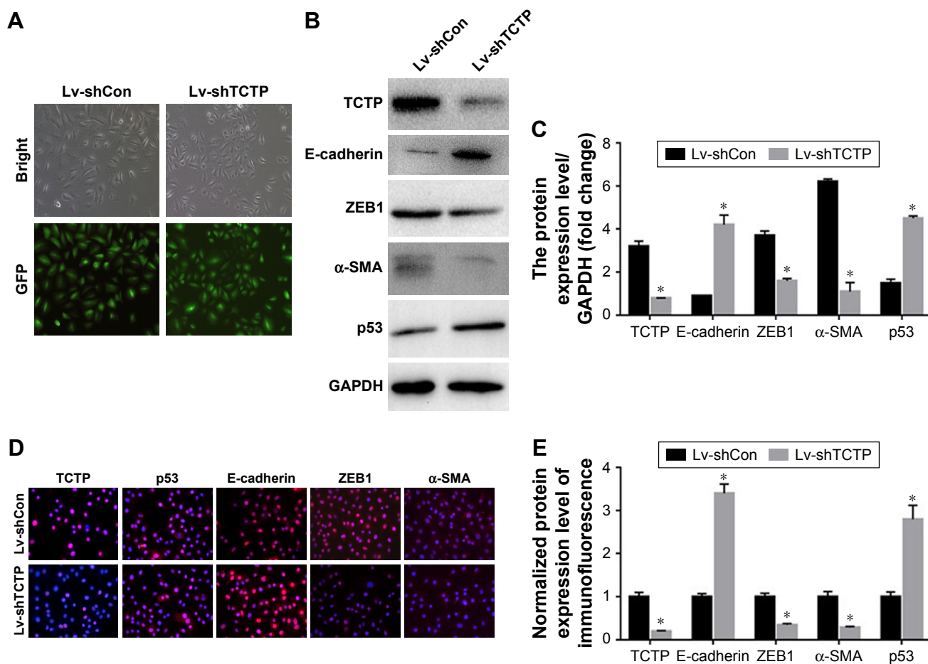
Figure 2 TCTP silencing in A549 cells using lentivirus-based short-hairpin RNA (Lv-shTCTP1).
