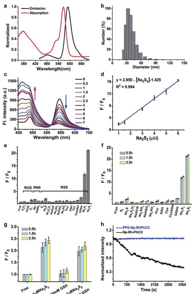
Fig. 3 (a) Absorption and fluorescence spectra of Np-RhPhCO ( 5 \mu\text{M} ) in MeCN/PBS ( v/v = 4 : 6 , PBS 25 \text{ mM} , pH 7.4 ) buffer solution at 37^\circ\text{C} . (b) Average hydrodynamic size of PPG-Np-RhPhCO measured by dynamic light scattering. (c) Fluorescence spectra of PPG-Np-RhPhCO ( 4.8 \mu\text{M} ) in the presence of various concentrations of \text{Na}_2\text{S}_2 ( 0, 0.5, 1.0, 1.5, 2.0, 2.5, 3.0, 5.0, 6.0, and 7.0 \mu\text{M} , respectively) in PBS buffer (pH 7.4 ) at 37^\circ\text{C} . \lambda_{\text{ex}} = 420 \text{ nm} . (d) Plot of fluorescence intensity ratio ( I_{486}/I_{594} ) changes as a function of \text{Na}_2\text{S}_2 concentration in PBS buffer (pH 7.4 ) at 37^\circ\text{C} . F and F_0 represent the fluorescence intensity ratio ( I_{486}/I_{594} ) in the presence and absence of \text{Na}_2\text{S}_2 , respectively. (e) Ratiometric fluorescence changes of PPG-Np-RhPhCO ( 4.8 \mu\text{M} ) in the presence of 7 \mu\text{M} \text{Na}_2\text{S}_2 and other biomolecules ( 1 \text{ mM} glutathione, 50 \mu\text{M} hypochloric acid, 50 \mu\text{M} GSSH/CysSSH, 30 \mu\text{M} \text{Na}_2\text{S}_4 , and 200 \mu\text{M} for other analytes). (f) Ratiometric fluorescence changes of PPG-Np-RhPhCO ( 4.8 \mu\text{M} ) in the presence of 7 \mu\text{M} \text{Na}_2\text{S}_2 and other RSS ( 5 \text{ mM} glutathione, 50 \mu\text{M} GSSH/CysSSH, 30 \mu\text{M} \text{Na}_2\text{S}_4 , and 200 \mu\text{M} for other analytes) after incubation for 0.5 \text{ h} , 1.5 \text{ h} , and 2.5 \text{ h} , respectively. (g) Ratiometric fluorescence changes of PPG-Np-RhPhCO ( 4.8 \mu\text{M} ) in the presence of 1 \mu\text{M} \text{Na}_2\text{S}_2 , 10 \text{ mM} GSH, and the mixture of 1 \mu\text{M} \text{Na}_2\text{S}_2 and 10 \text{ mM} GSH after incubation for 0.5 \text{ h} , 1.5 \text{ h} , and 2.5 \text{ h} , respectively. F and F_0 represent the fluorescence intensity ratio ( I_{486}/I_{594} ) in the presence and absence of analytes, respectively. Measurement conditions: \lambda_{\text{ex}} = 420 \text{ nm} , PBS (pH 7.4 ) buffer, 37^\circ\text{C} . (h) Normalized time-dependent emission profile of PPG-Np-RhPhCO ( 4.8 \mu\text{M} ) and Np-RhPhCO ( 5 \mu\text{M} ) with continuous irradiation for 1 \text{ h} in PBS (pH = 7.4 , 1\% MeCN) at 37^\circ\text{C} using a Xe-lamp at 420 \text{ nm} .
