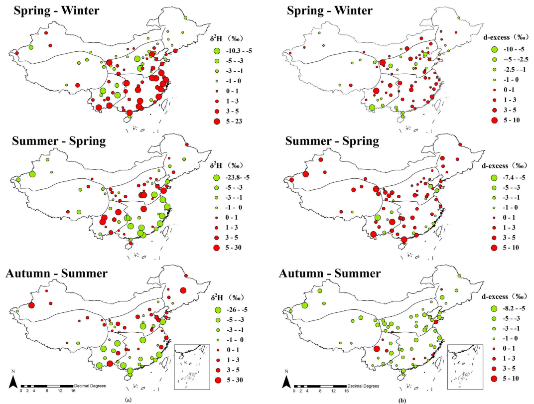
Figure 4. Seasonal differences of \delta^2\text{H} and d\text{-excess} values in tap water, expressed in circles with different sizes and two colors, green represents value decreasing and red represents increasing, circle size represents the magnitude of seasonal variation. (All of the items were generated with Arcgis 9.3, https://www.arcgis.com/features/index.html ).
